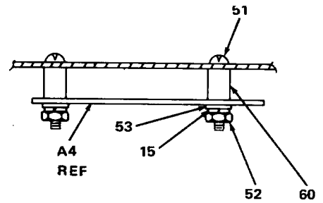
SECTION J-J (ROTATED 90° CW)
