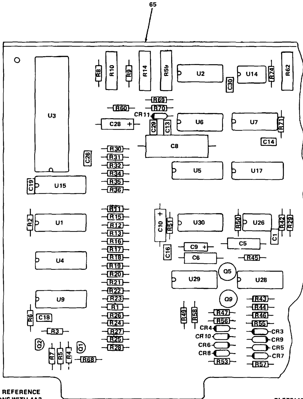
Figure 46. Operation Site (Remote) Modem Circuit Card Assembly (4A3) (Sheet 1 of 3).
