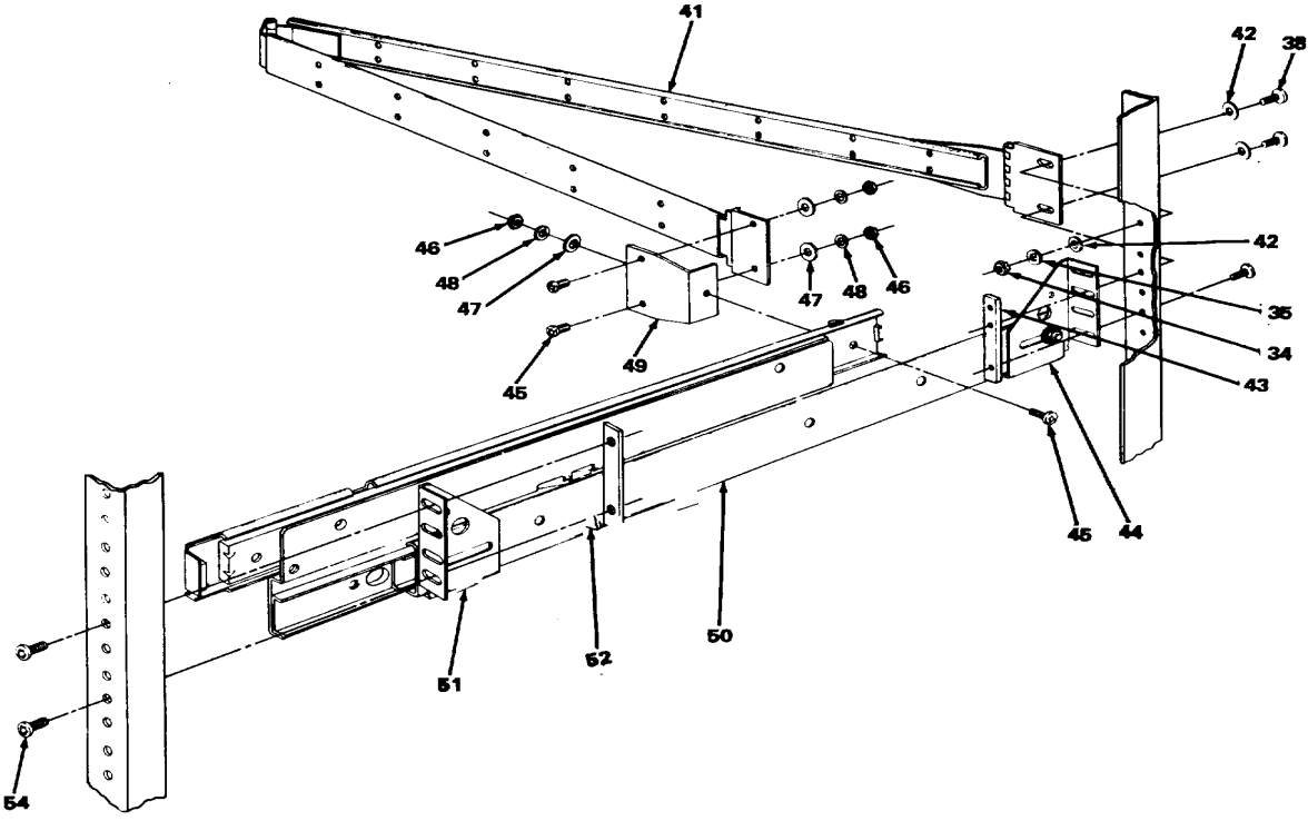
DETAIL L
