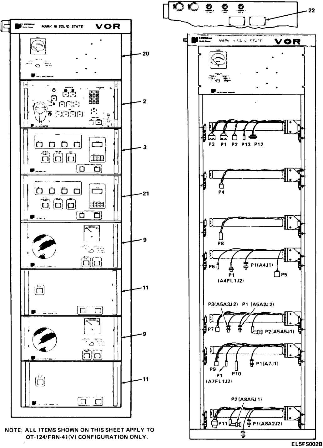
Figure 2. Transmitter Group (Unit 1) OT-117/FRN-41(V) and OT-124/FRN-41-(V) (Sheet 3 of 3).
