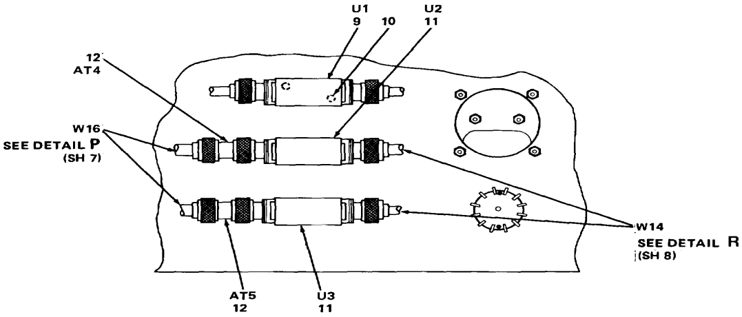
PARTIAL REAR VIEW OF FRONT PANEL
