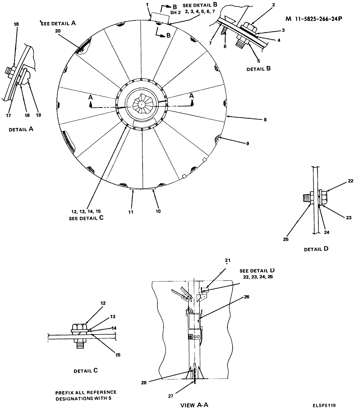
Figure 47. Shelter S-597/FRN-41(V) (Sheet 1 of 2)
