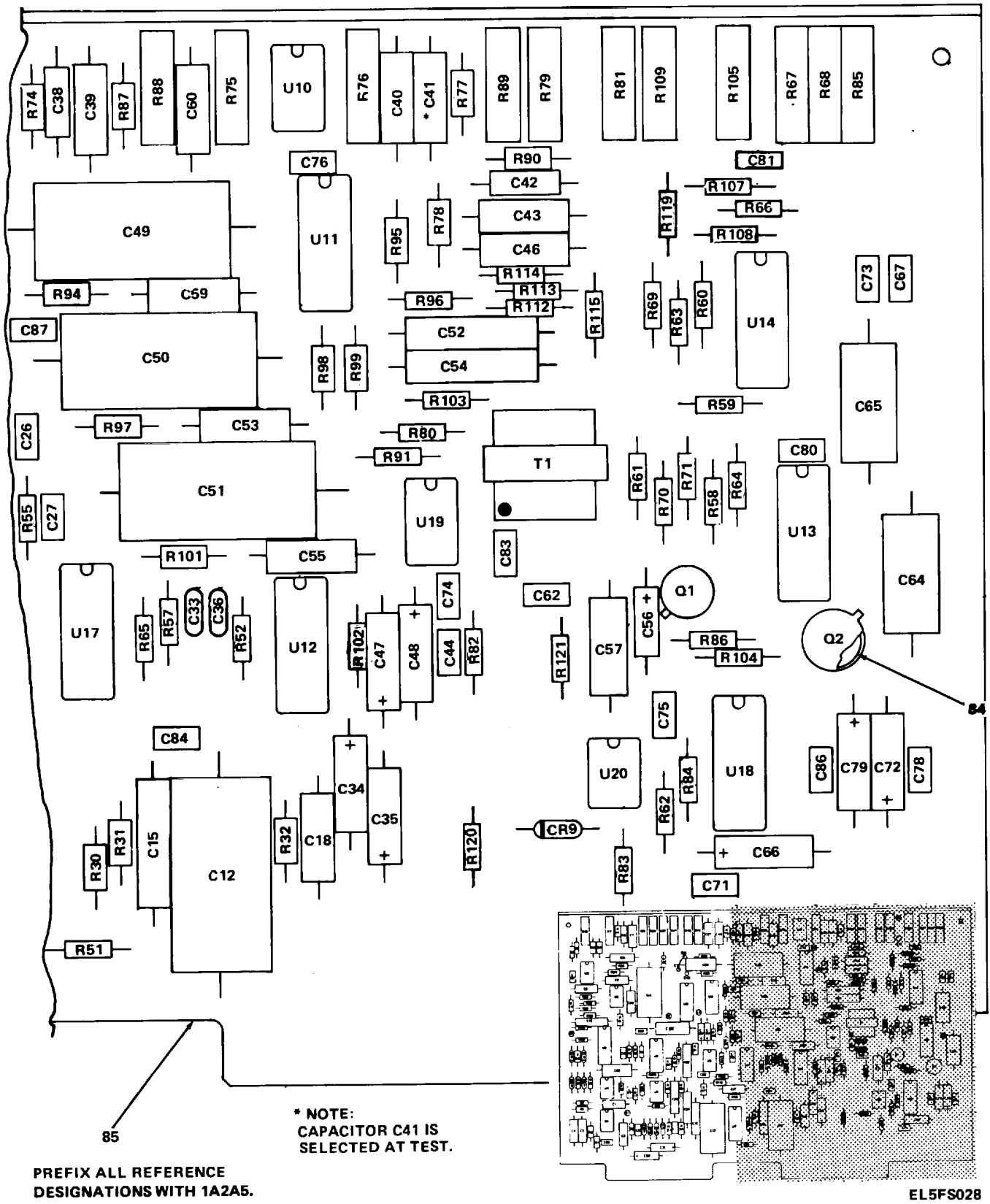
Figure 9. Transmitter/ Receiver Voice Buffer Circuit Card Assembly (1A2A5) (Sheet 2 of 3)
