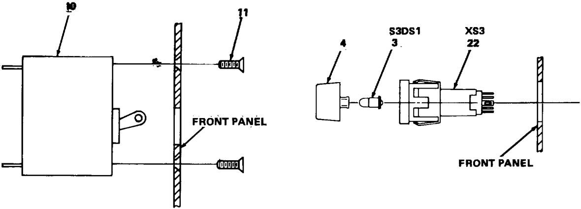
DETAIL C
