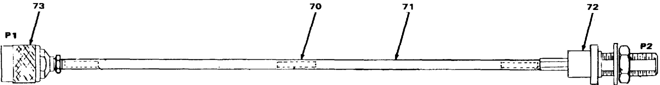
DETAIL P ITEM 70 (W16) CONSISTS OF ITEMS 71, 72 & 73
