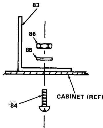
DETAIL L
