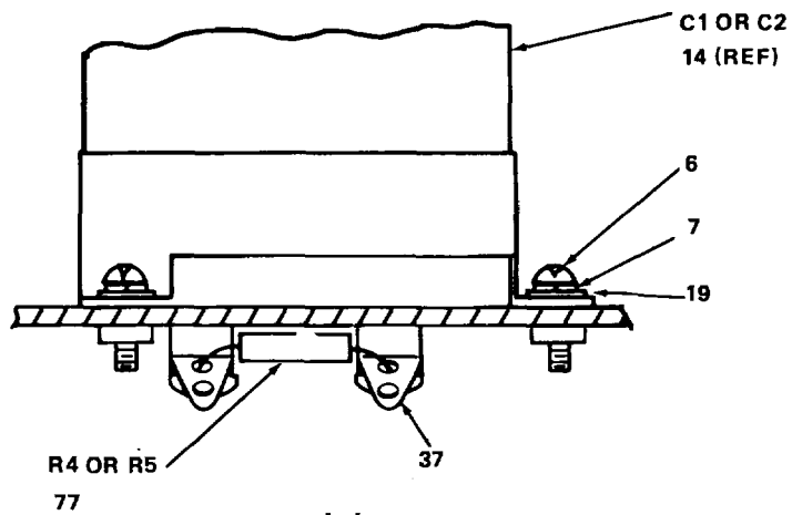
SECTION L-L
