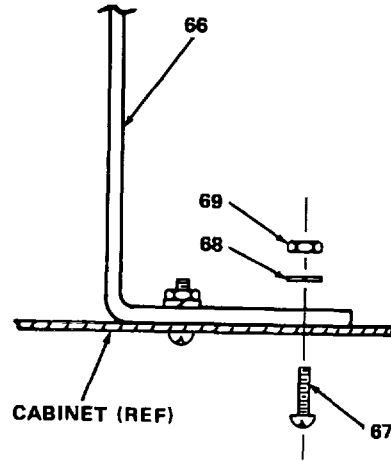
DETAIL J
