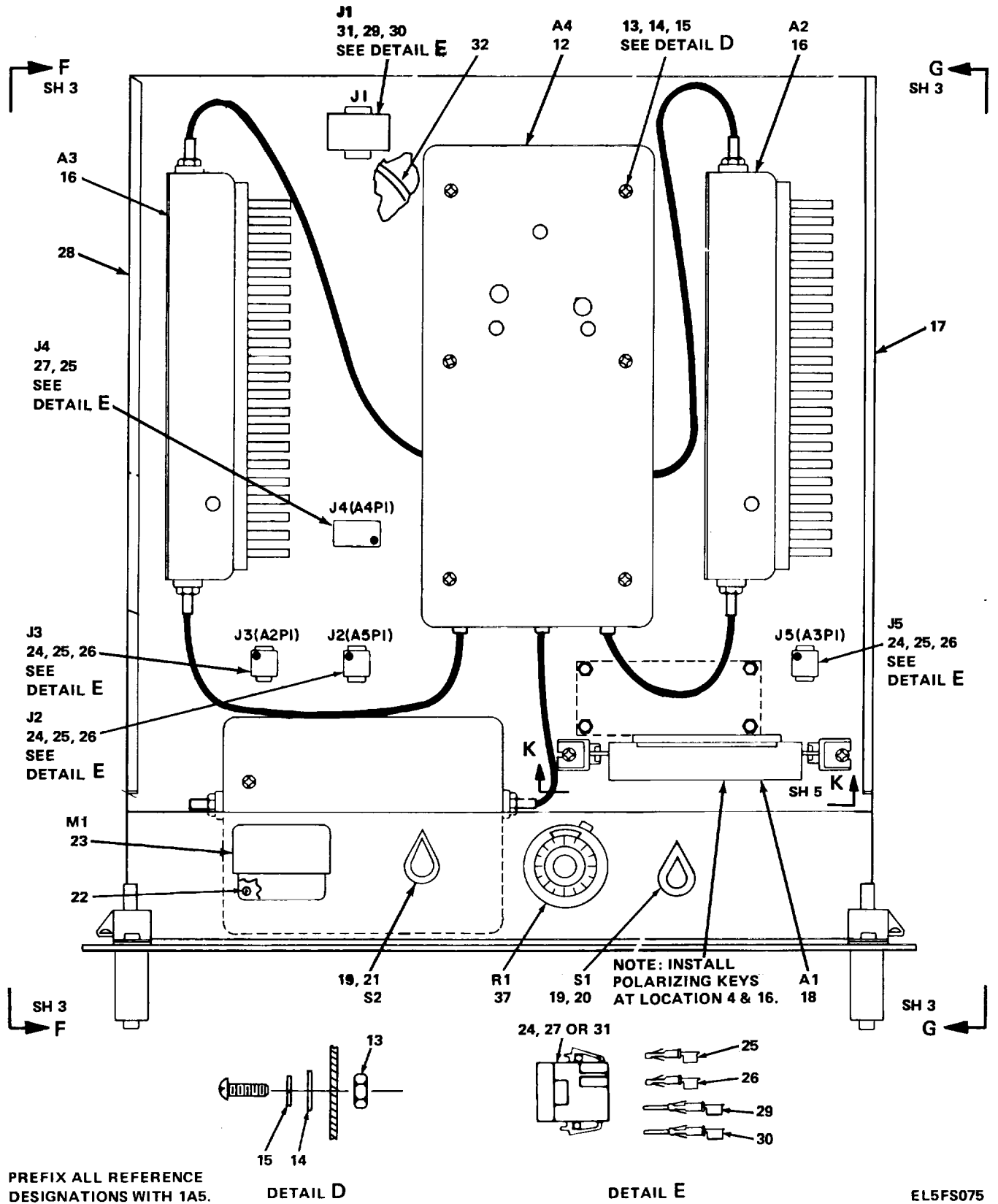
Figure 30. Sideband Transmitter (1A5/1A8) T-1395/FRN-41(V) (Sheet 2 of 5).
