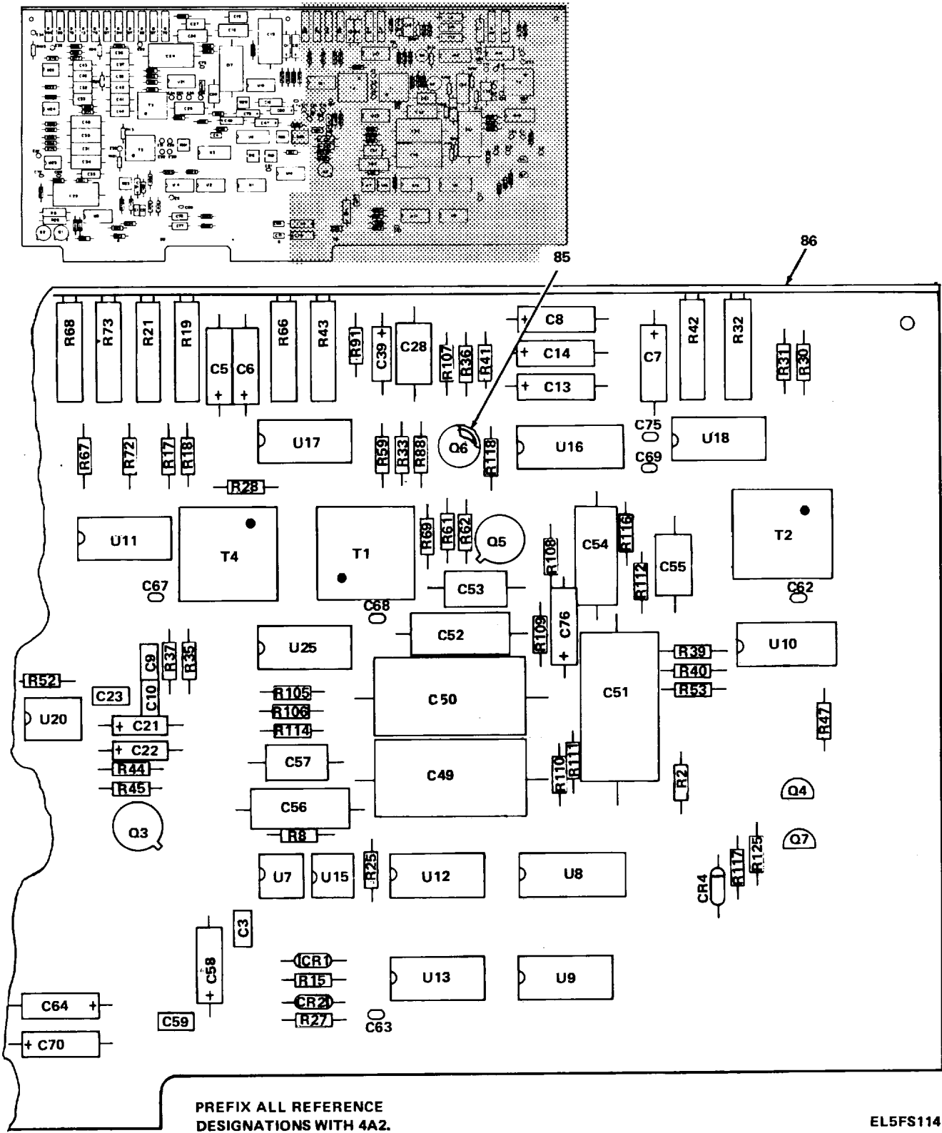
Figure 45. Operation Voice Buffer Circuit Card Assembly (4A2) (Sheet 2 of 3).
