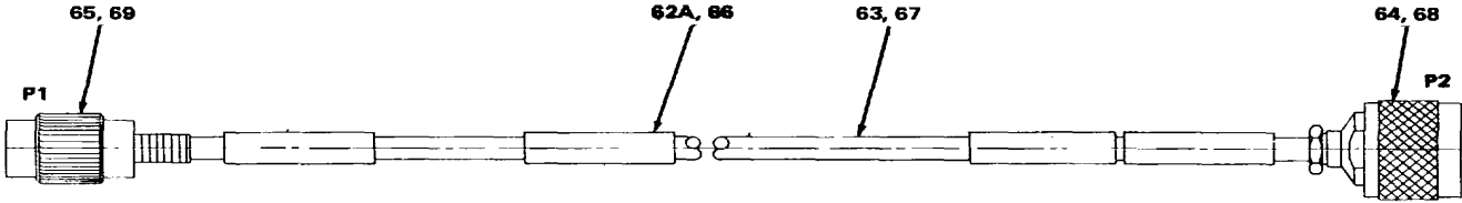
DETAIL N ITEM 62A (W3) CONSISTS OF ITEMS 63, 64 & 65 ITEM 66 (W5) CONSISTS OF ITEMS 67, 68 & 69
