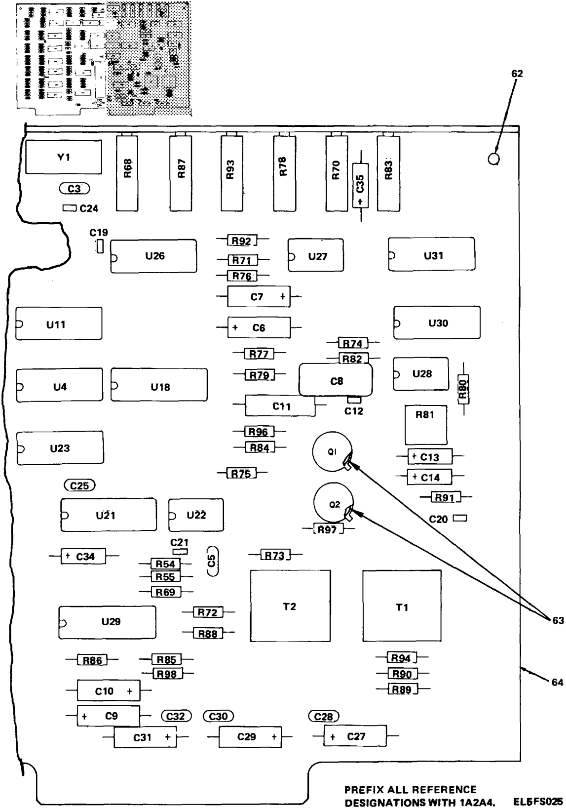
Figure 8. Status Transformer (Local Modem Circuit Card Assembly(1A2A24) (Sheet 2 of 3).
