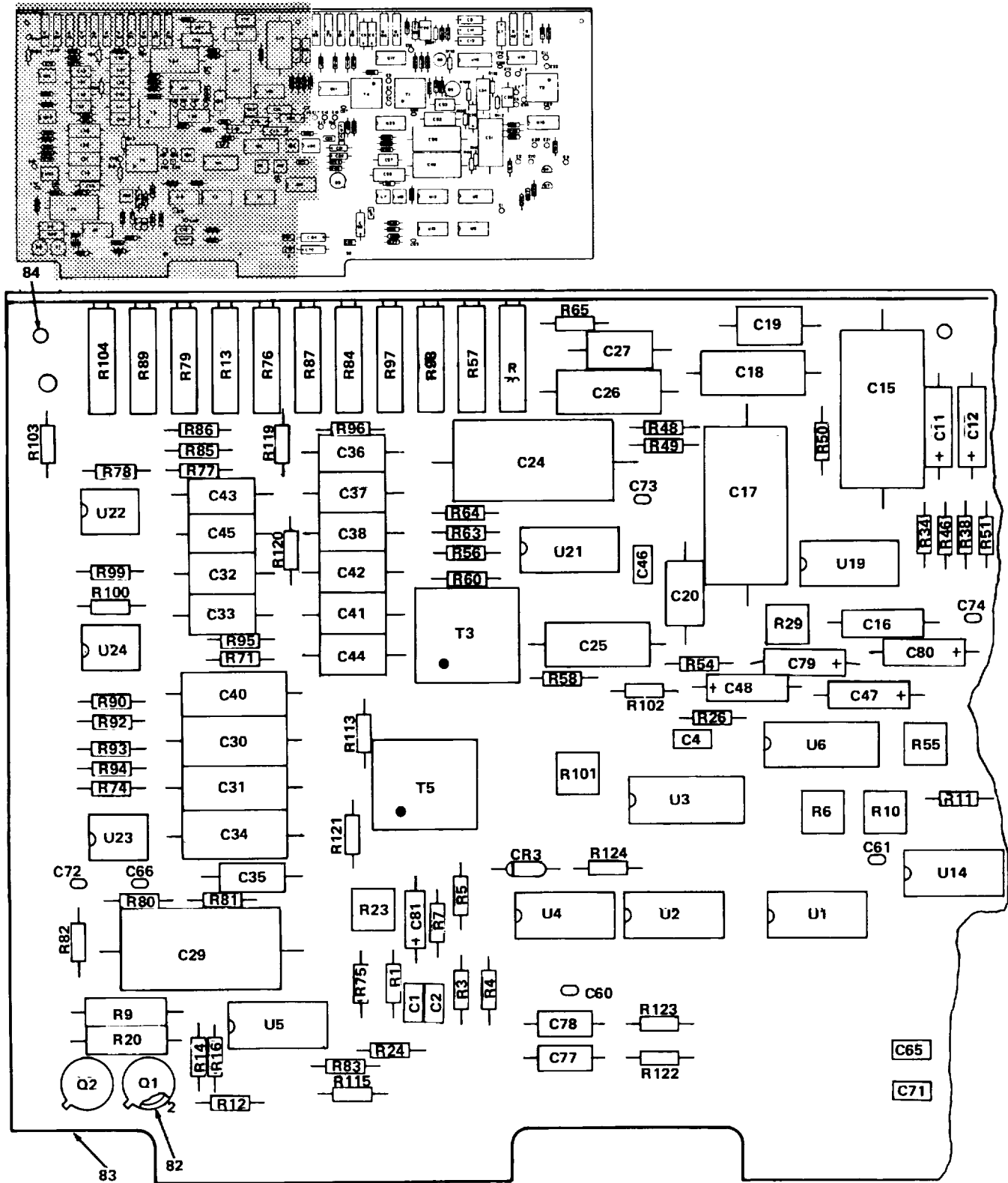
Figure 45. Operation Voice Buffer Circuit Card Assembly (4A2) (Sheet 1 of 31).
