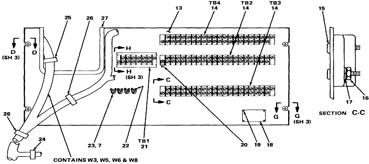
REAR VIEW OF REAR PANEL
