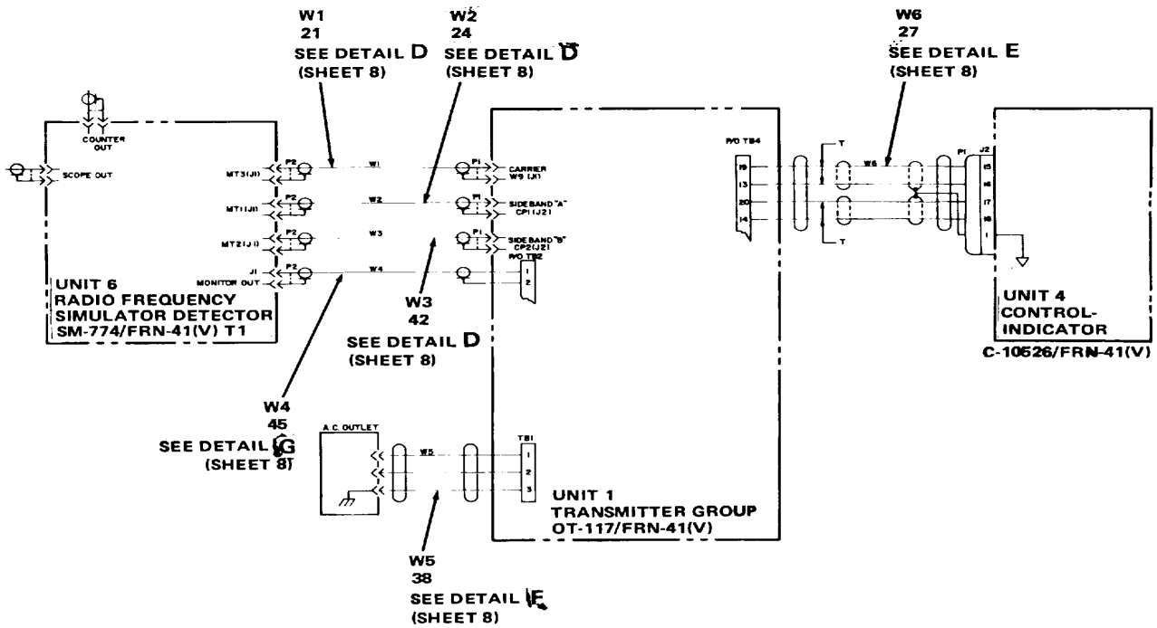
INTERCONNECTING DIAGRAM
