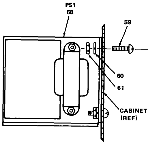
DETAIL H
