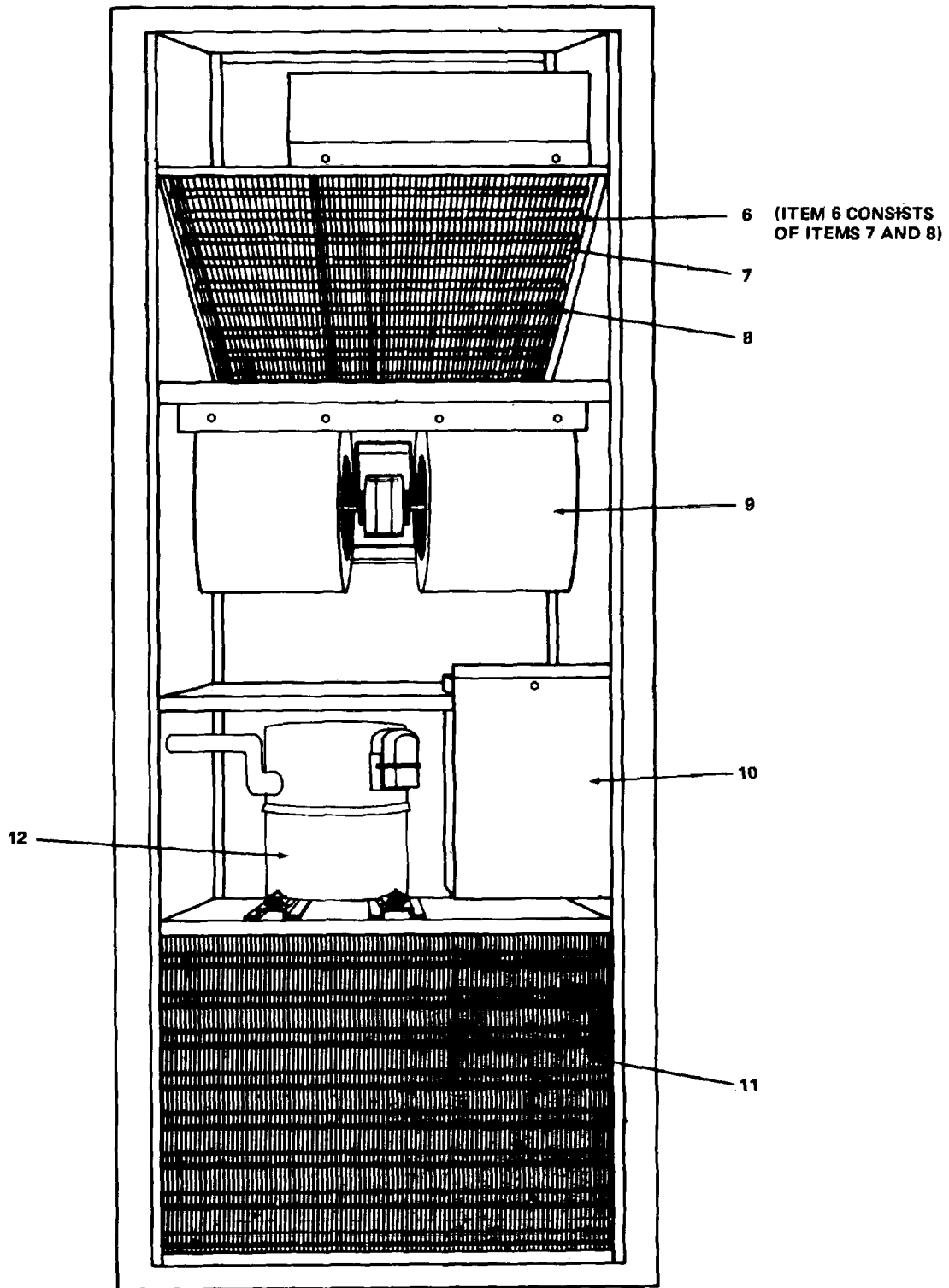
REAR VIEW
