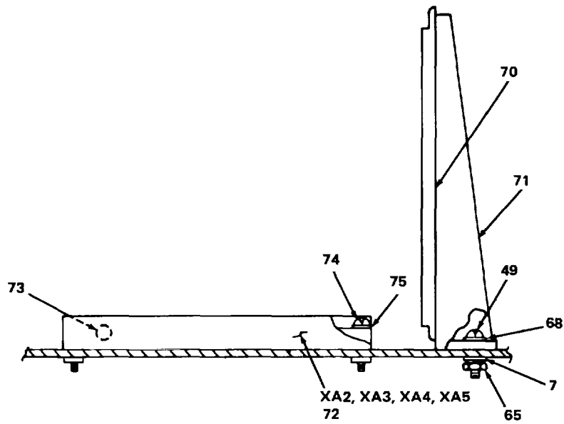
SECTION J-J
