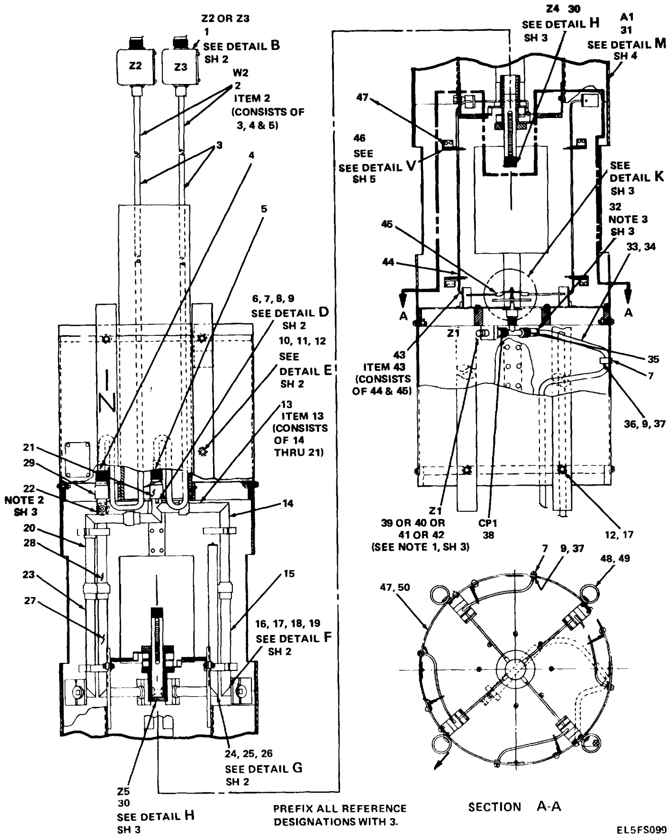
Figure 41. Antenna (Unit S) AS-SSS2FRN-41(V) (Sheet 1 of 5).
