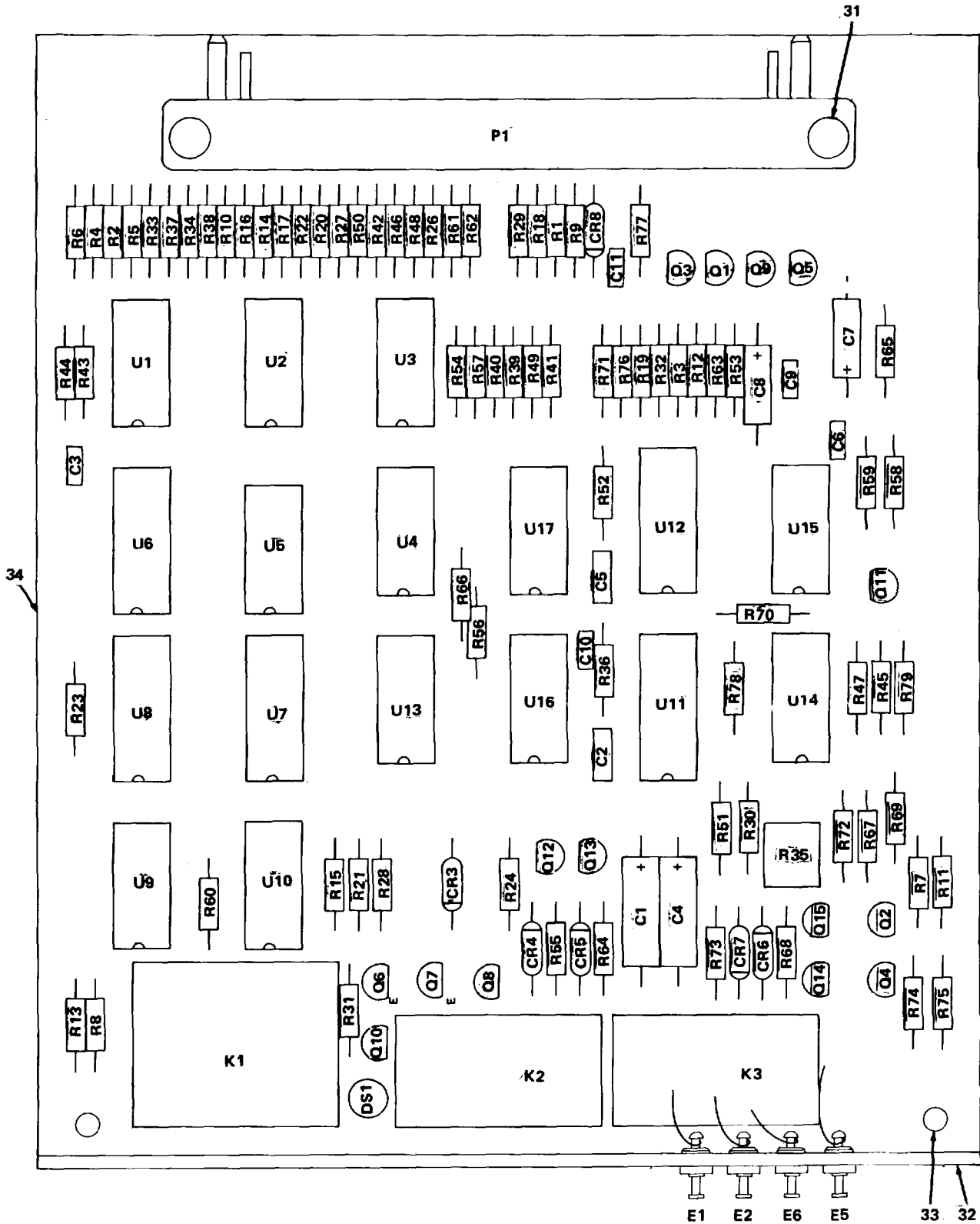
Figure 6. Alarm and Transfer Circuit Card Assembly (1A2A2) (Sheet 1 of 2)
