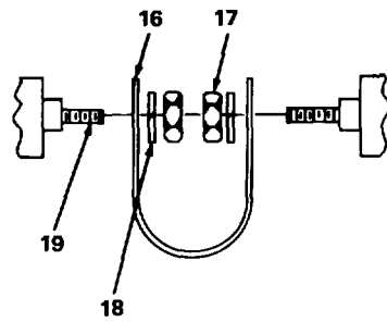
DETAIL F
