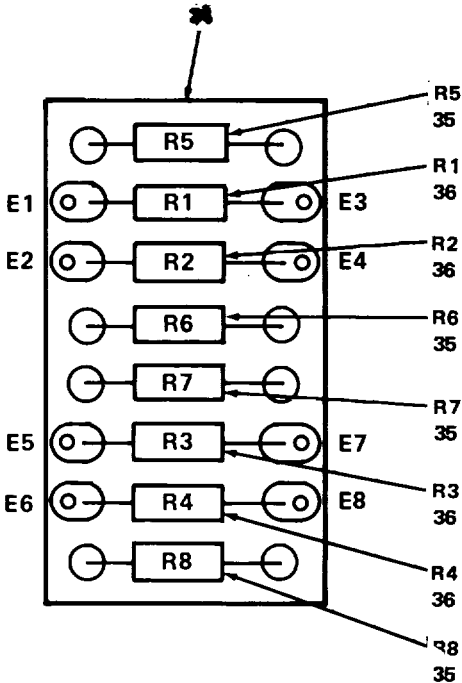
DETAIL H ITEM 33 (CONSISTS OF ITEMS 34, 35 & 36)
