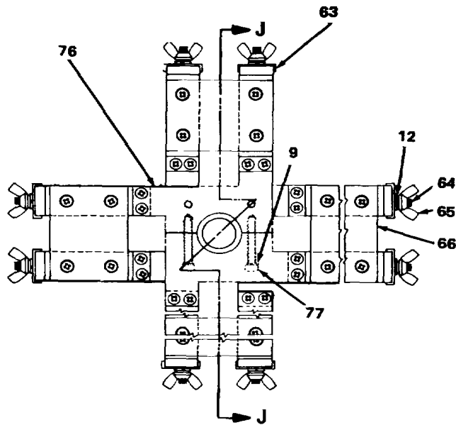
DETAIL H ITEM 30 (CONSISTS OF ITEMS 63 THRU 84)
