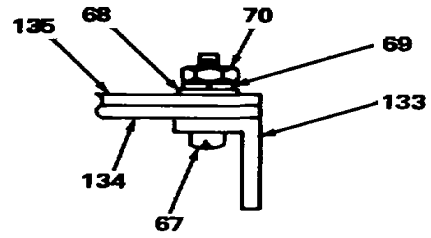
DETAIL V
