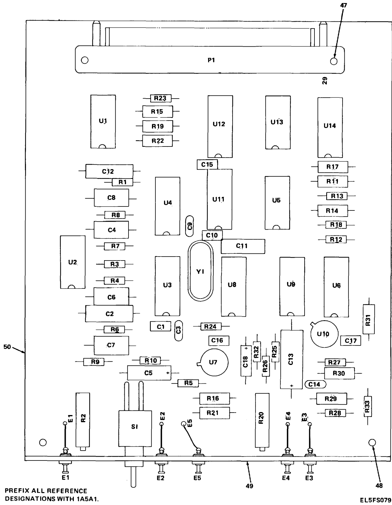
Figure 31. Reference and Subcarrier Generator Circuit Card Assembly (1A5A1/1A8A1) (Sheet 1 of 2).
