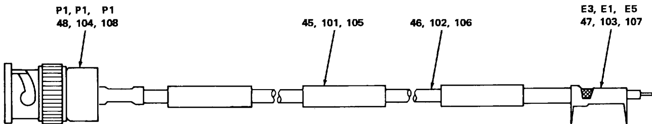
DETAIL G
