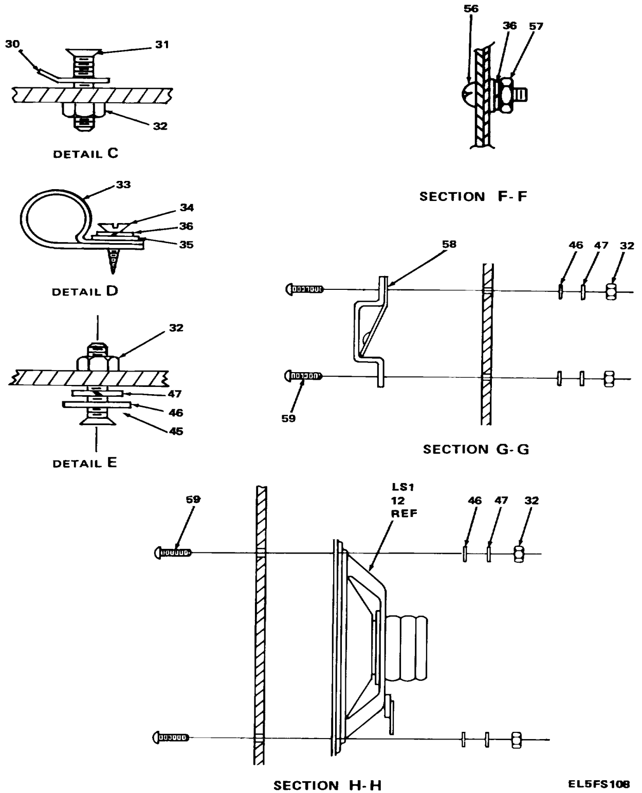
Figure 43. Control-Indicator (Unit 4) C-10526/FRN-41(V) (Sheet 3 of 5).
