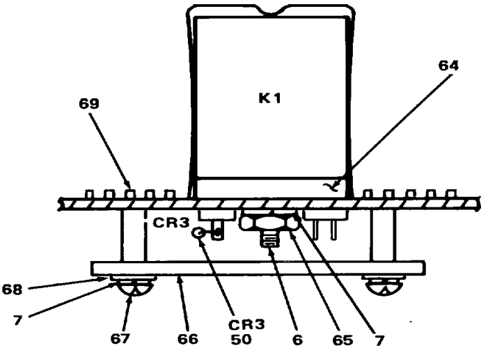
SECTION H-H (ROTATED 180° CW)
