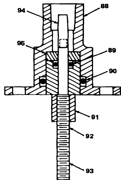
DETAIL L
