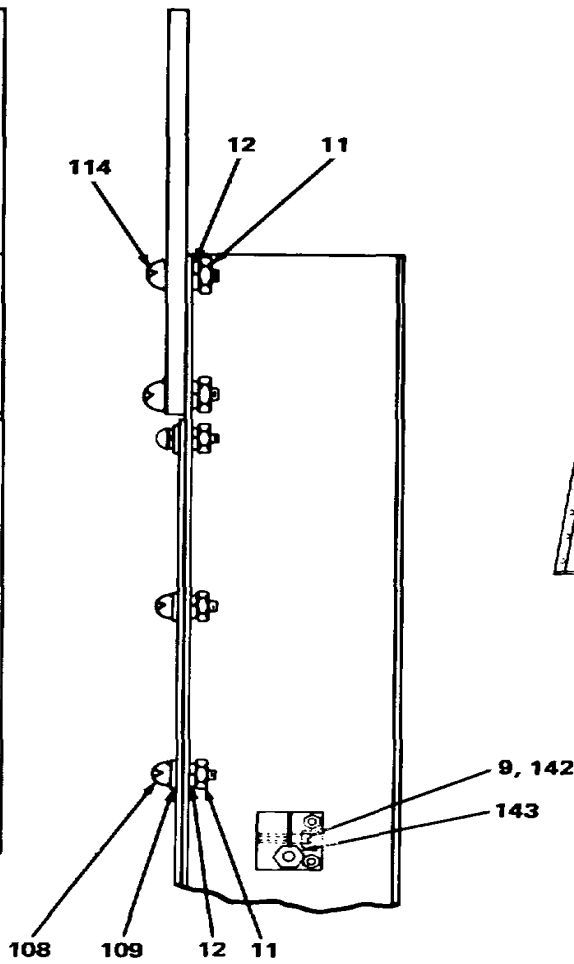
DETAIL W
