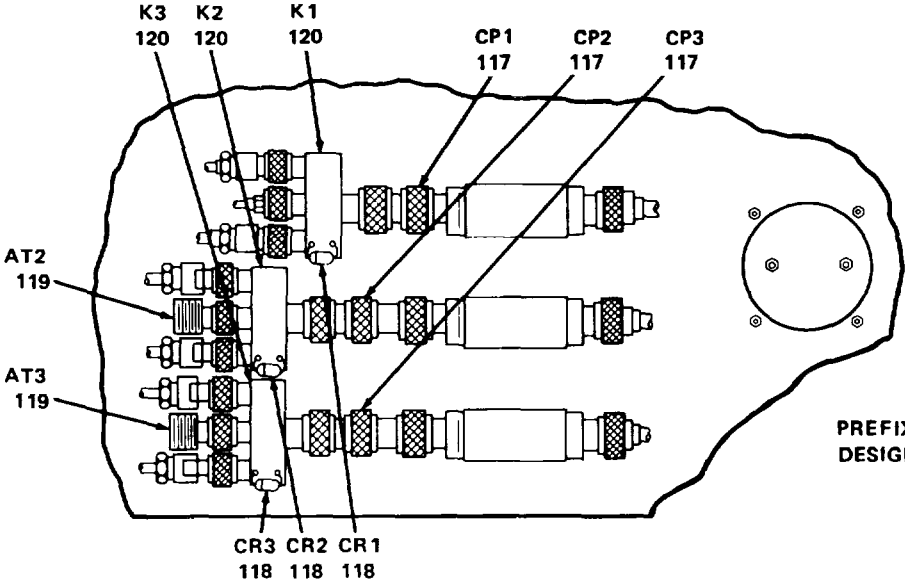
PARTIAL REAR VIEW OF FRONT PANEL
