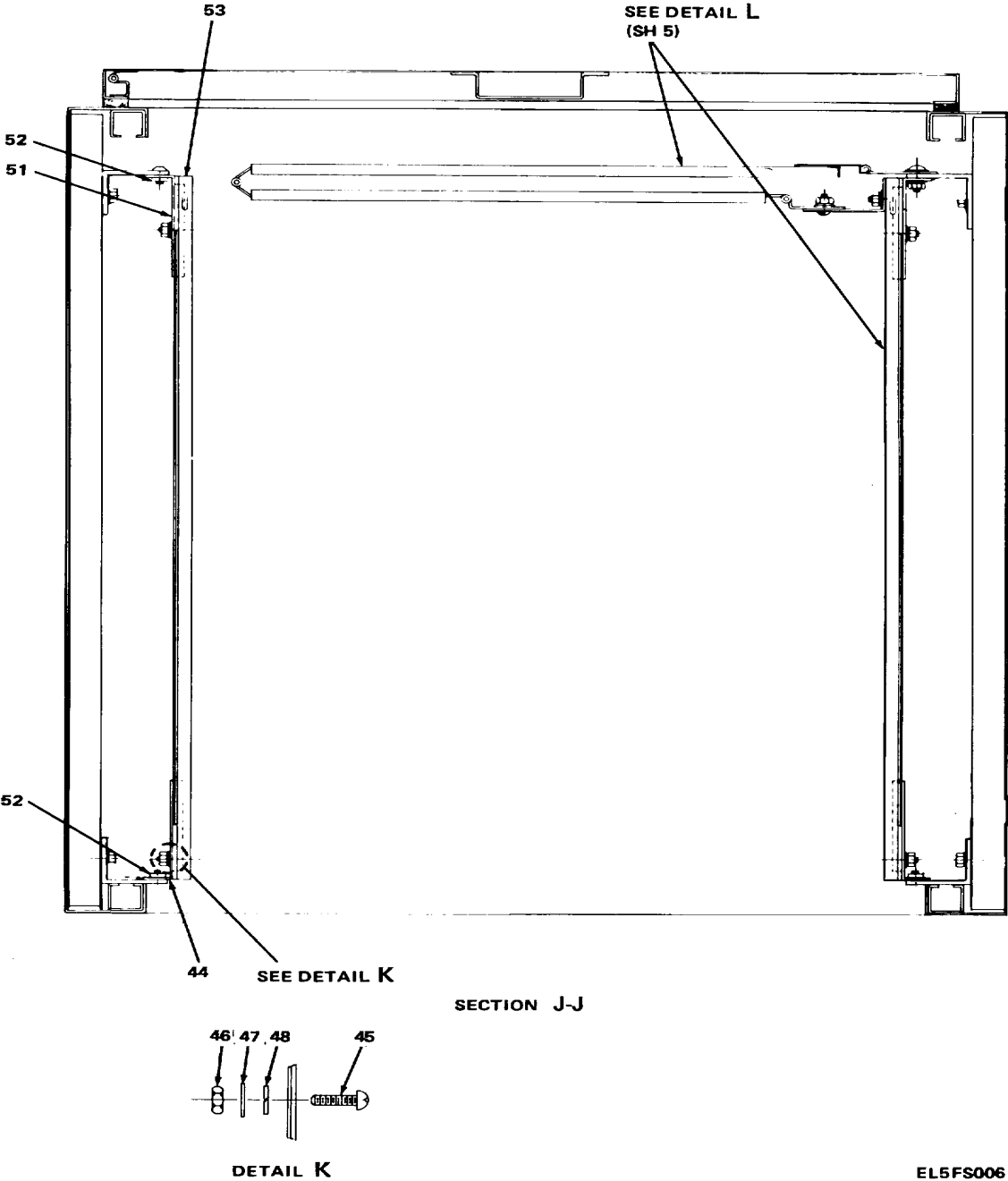
Figure 3. Electrical Equipment Rack (1A1) MT-6011/FRN-41(V) and MT-6134/FRN-41(V) (Sheet 4 of 11).
