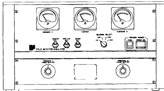
UNIT 6 RADIO FREQUENCY SIMULATOR DETECTOR SM-774/FRN-41(V) T1
