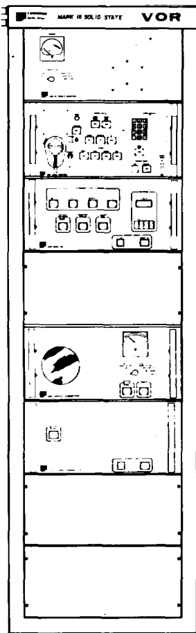
UNIT 1 TRANSMITTER GROUP OT-117/FRN-41(V)
