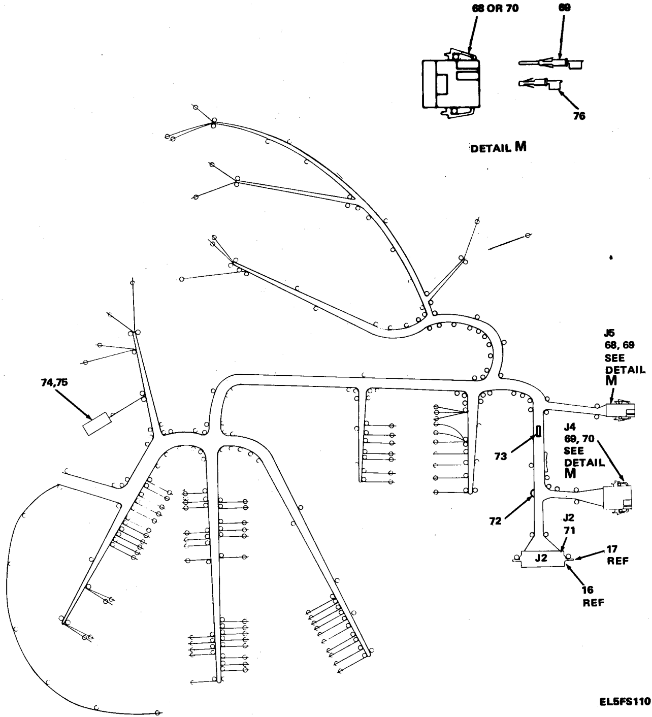
Figure 43. Control-Indicator (Unit 4) C-10526/FRN-41(V) (Sheet 5 of 5)
