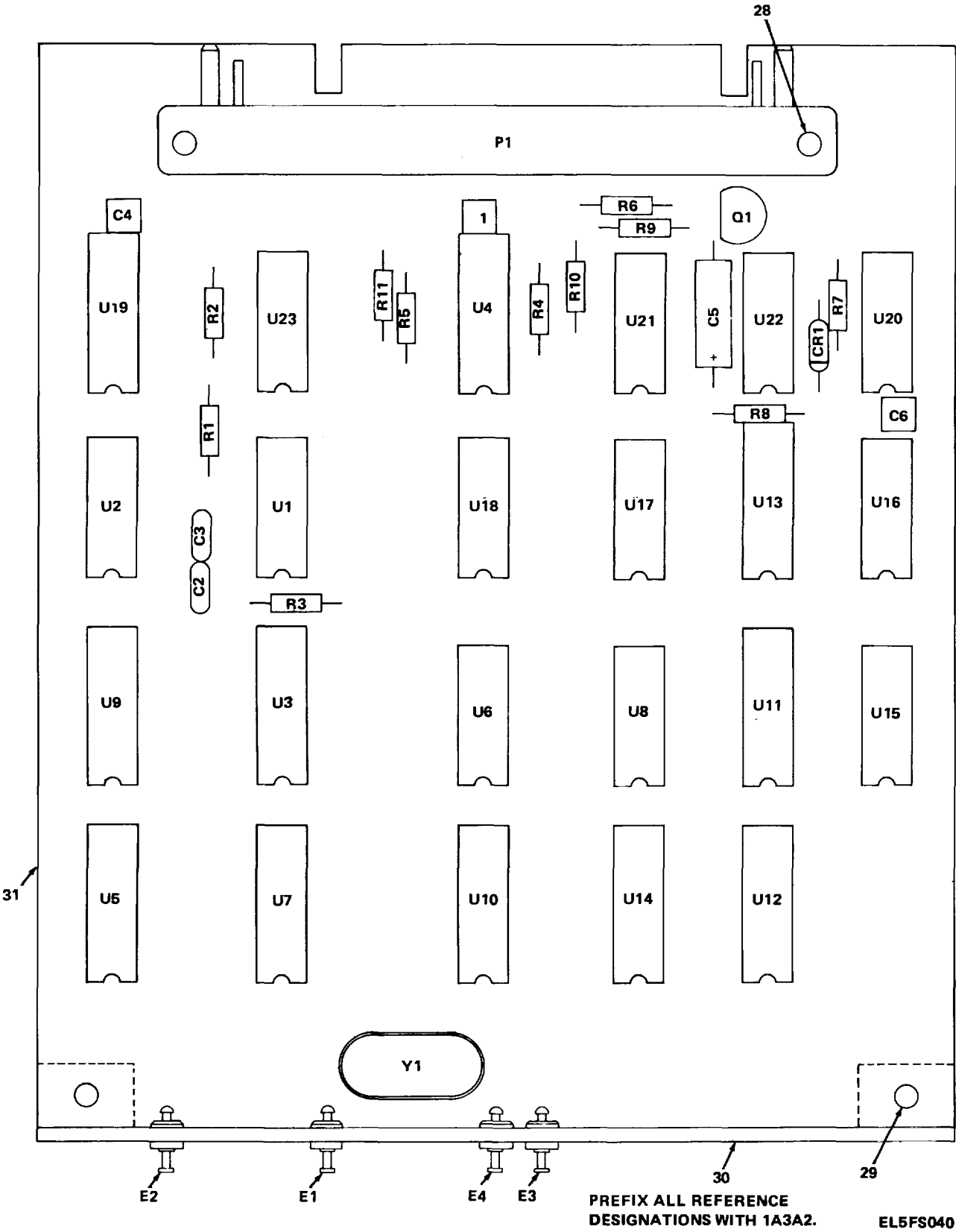
Figure 14. Phase Comparator Circuit Card Assembly (1A3A2/1A6A2/1A6A2) (Sheet 1 of 2)
