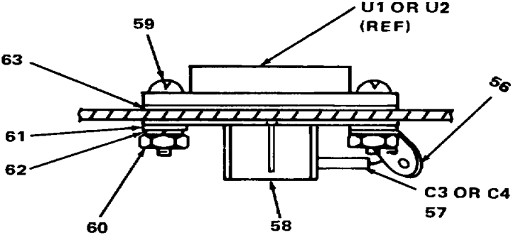
SECTION G-G (ROTATED 90° CW)
