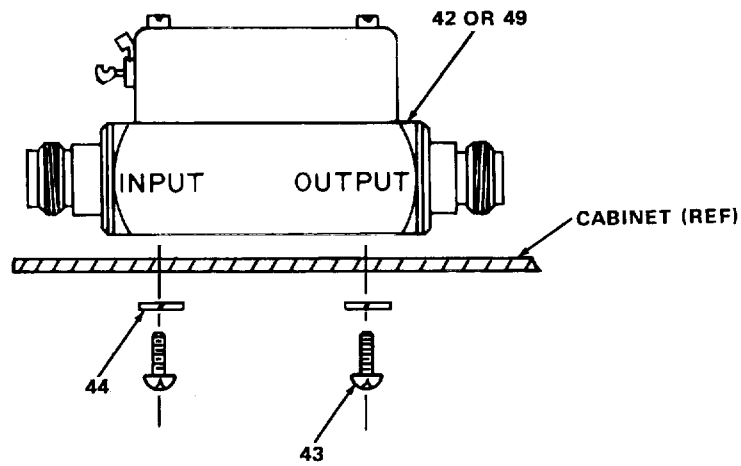
DETAIL F
