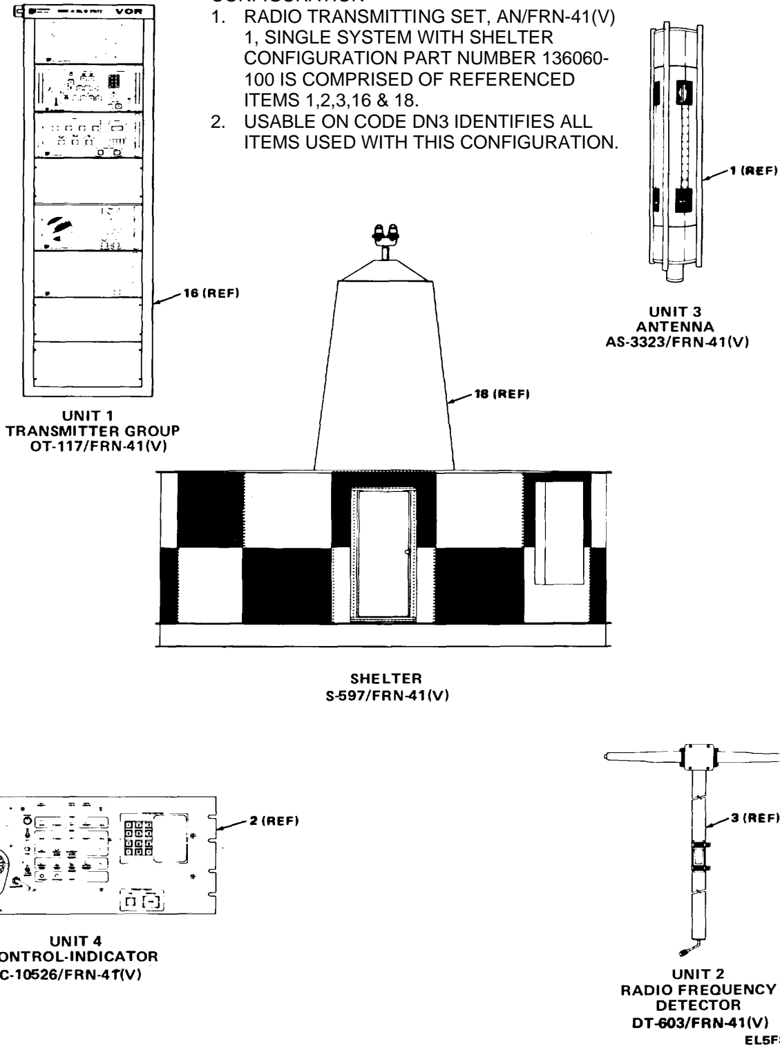
Figure 1. Radio Transmitting Set AN/FRN-41(V) 1,2,3 and 4 and Radio Transmitting Training Set AN/FRN-41(V) T1(Sheet 2 of 9).
