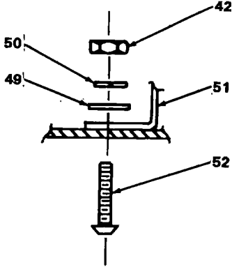
SECTION J-J
