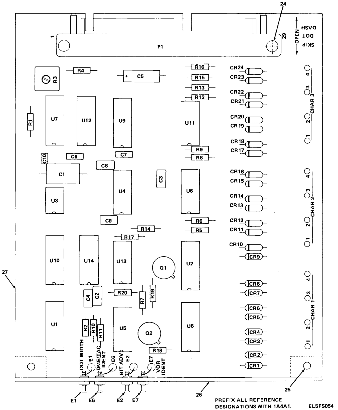
Figure 19. Ident Keyer Circuit Card Assembly (1A4A1/1A7A1) (Sheet 1 of 2).
