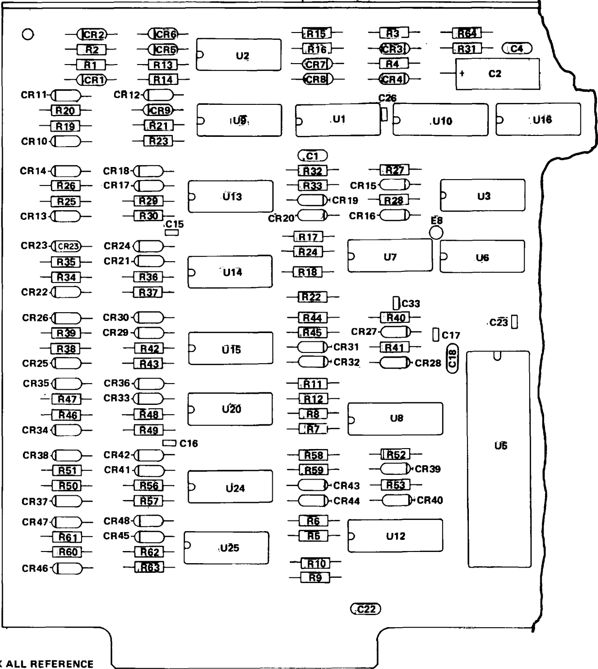
Figure 8. Status Transformer (Local) Modem Circuit Card Assembly (1A2A4 (Sheet 1 of 3).
