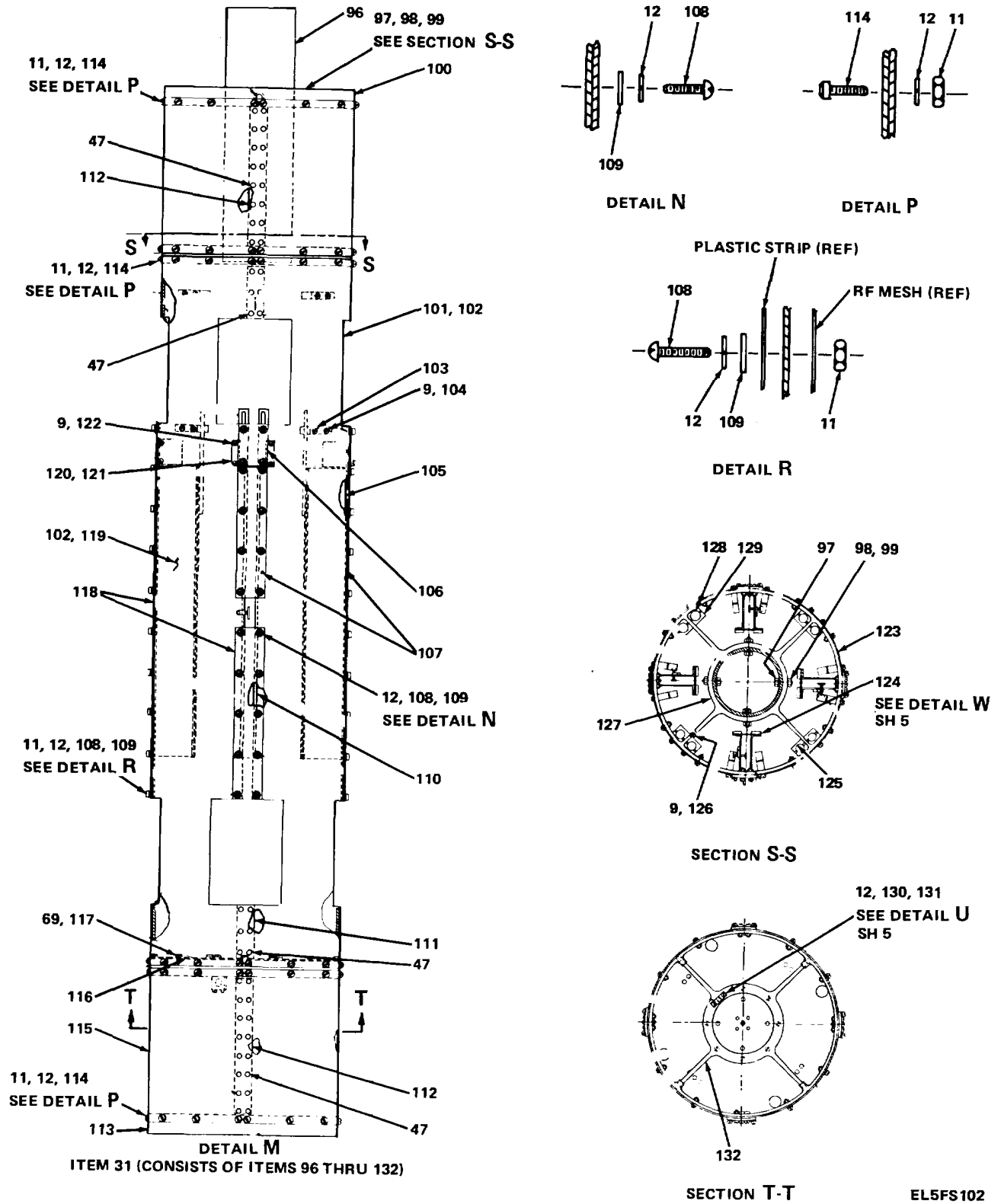
Figure 41. Antenna (Unit 3) AS-332/FRN-41(V) (Sheet 4 of 5)
