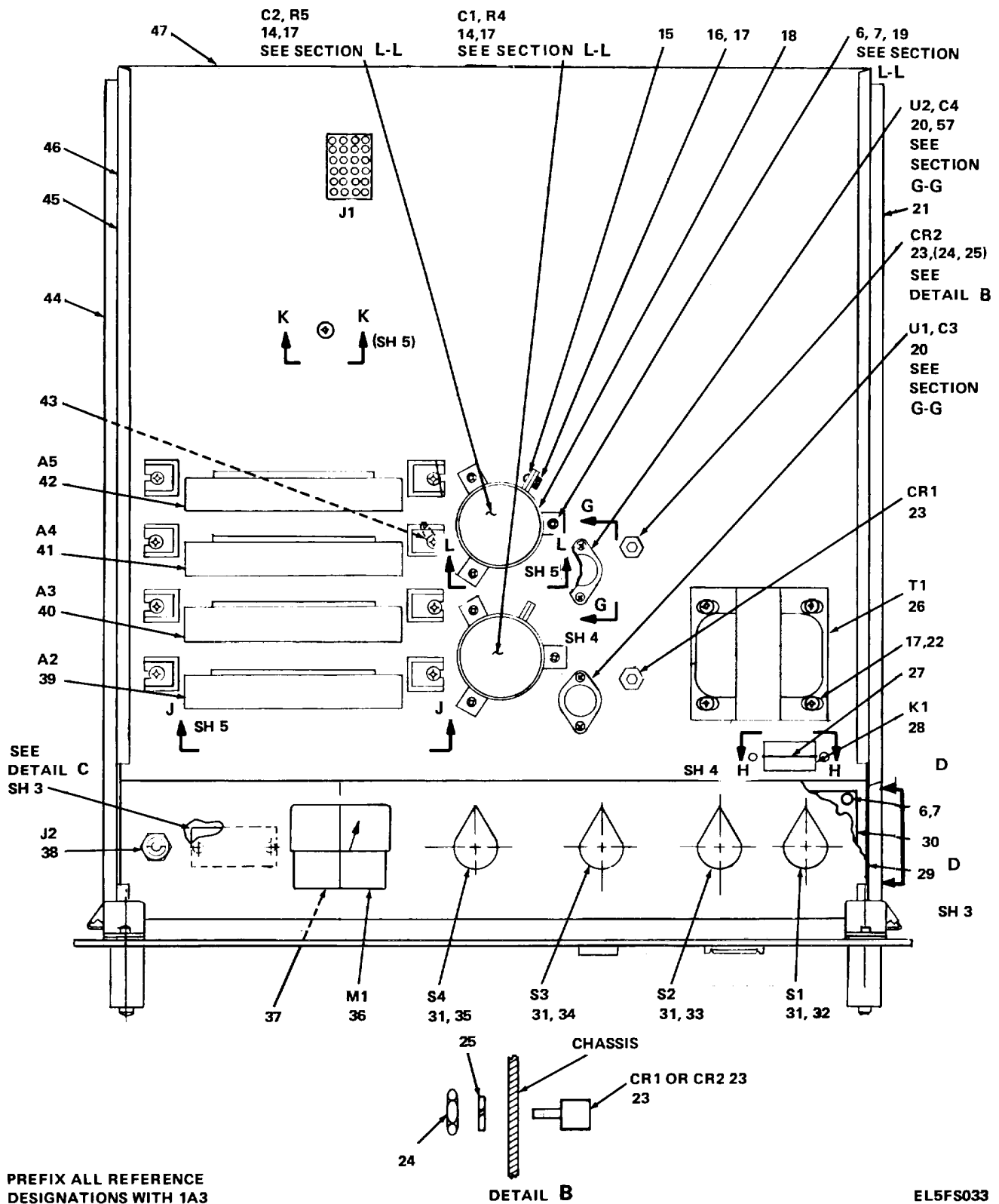
Figure 12. Phase Modulation Monitor (1A3)ID-2179/FRN-41(V) and (1A6) ID-2240/FRN-41(V) (Sheet 2 of 7)
