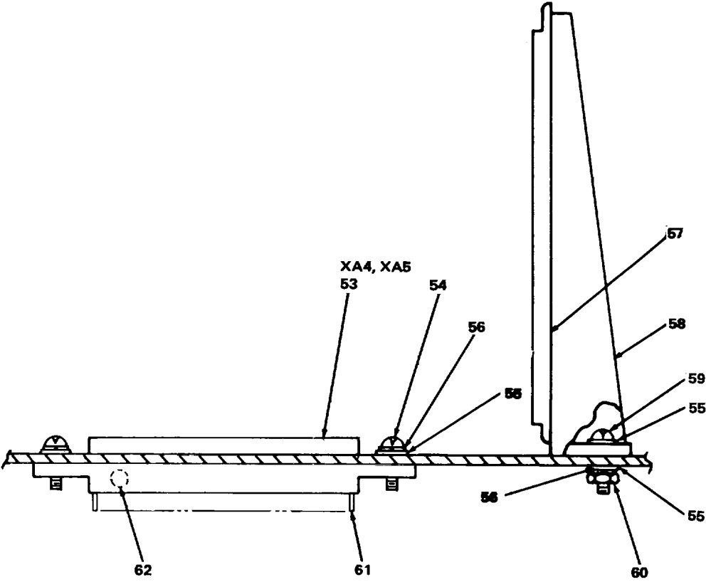
SECTION K-K
