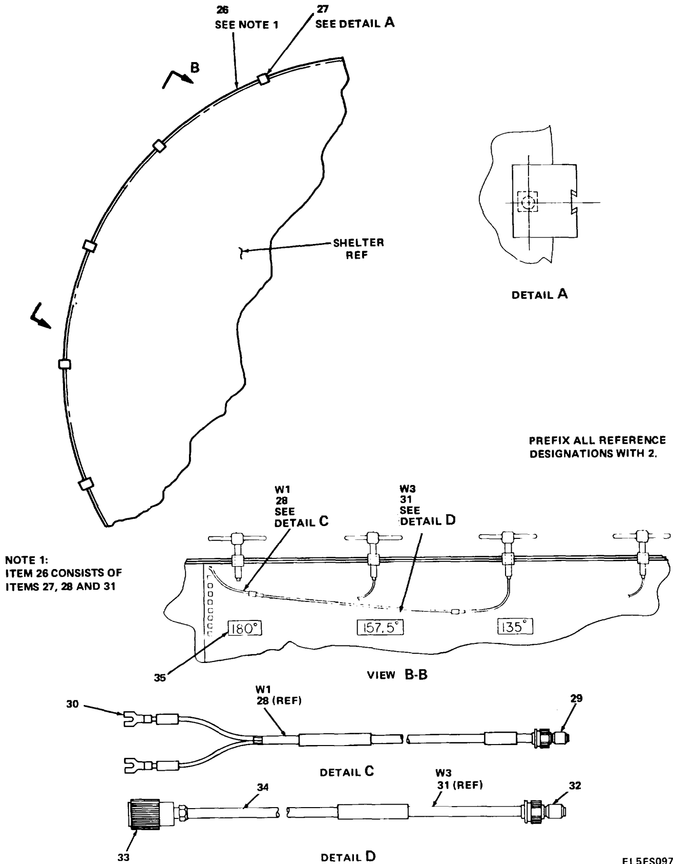
Figure 39. Radio Frequency Detector (Unit 2) DT-603/FRN-41(V) (Sheet 3 of 3).
