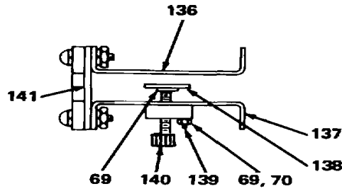
DETAIL V
