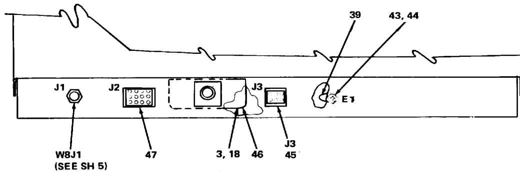
VIEW D-D (ROTATED 180° CW)
