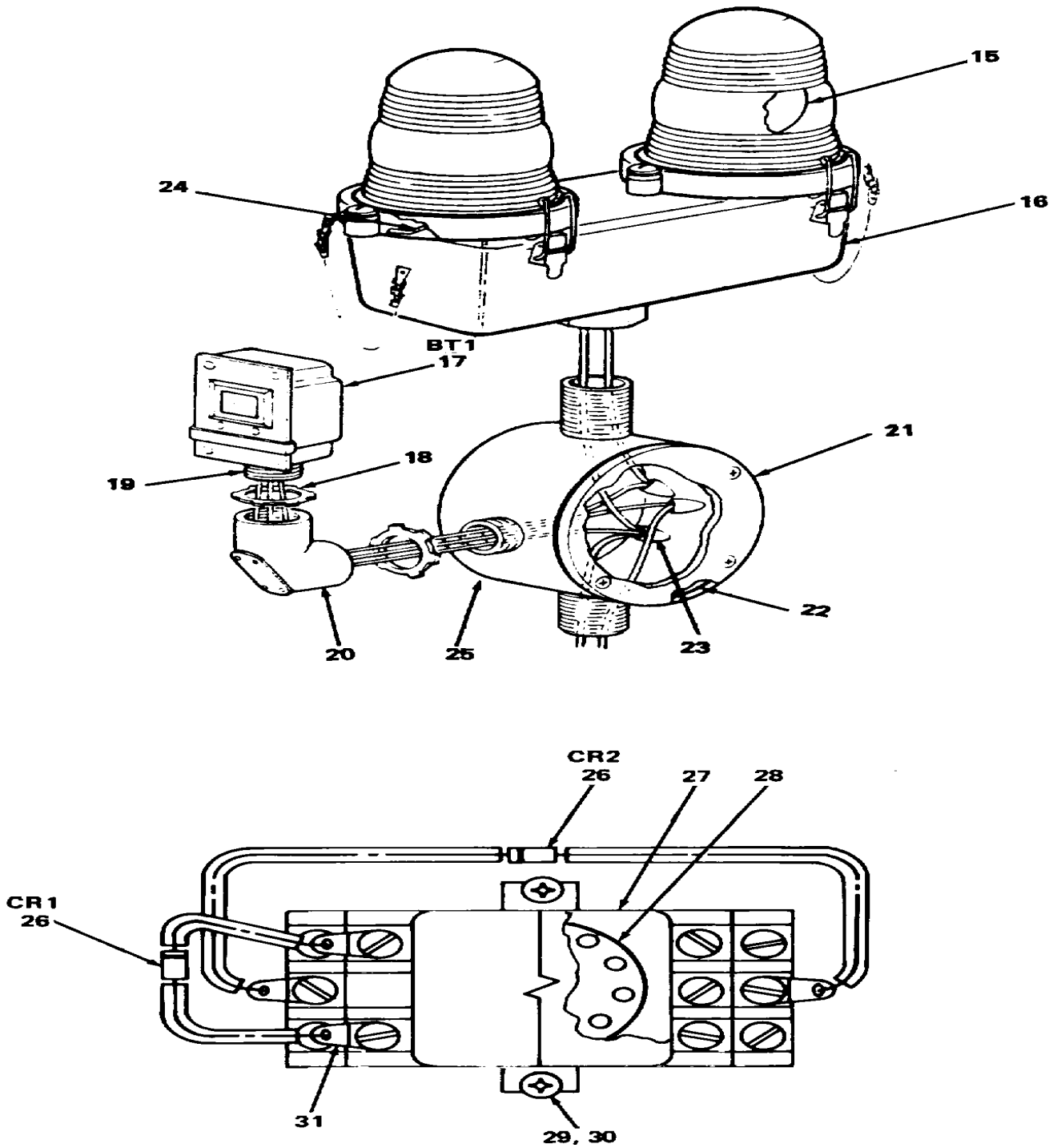
Figure 42. Radome Assembly (3A3) (Sheet 2 of 2)
