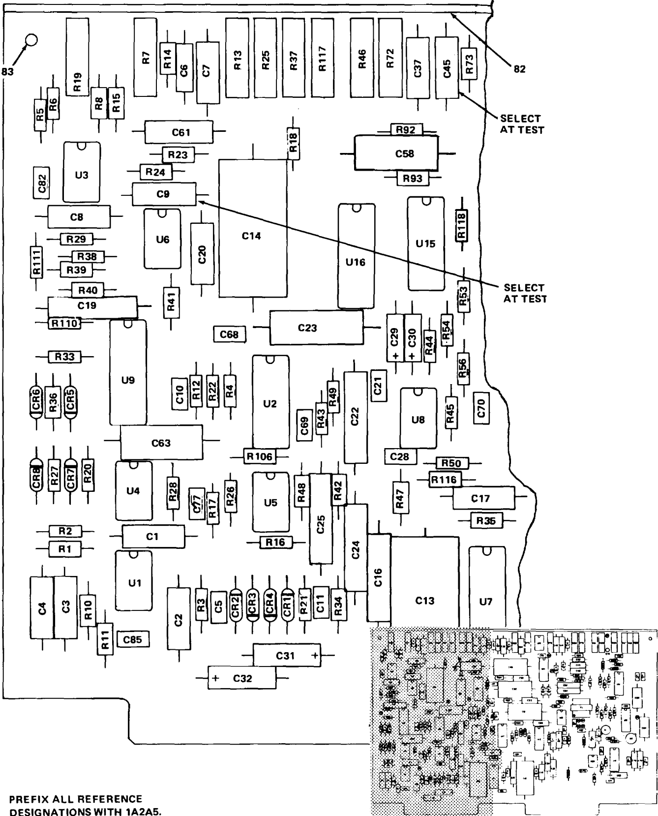
Figure 9. Transmitter/receiver voice buffer circuit card assembly (1A2A5) (Sheet 1 of 3).
