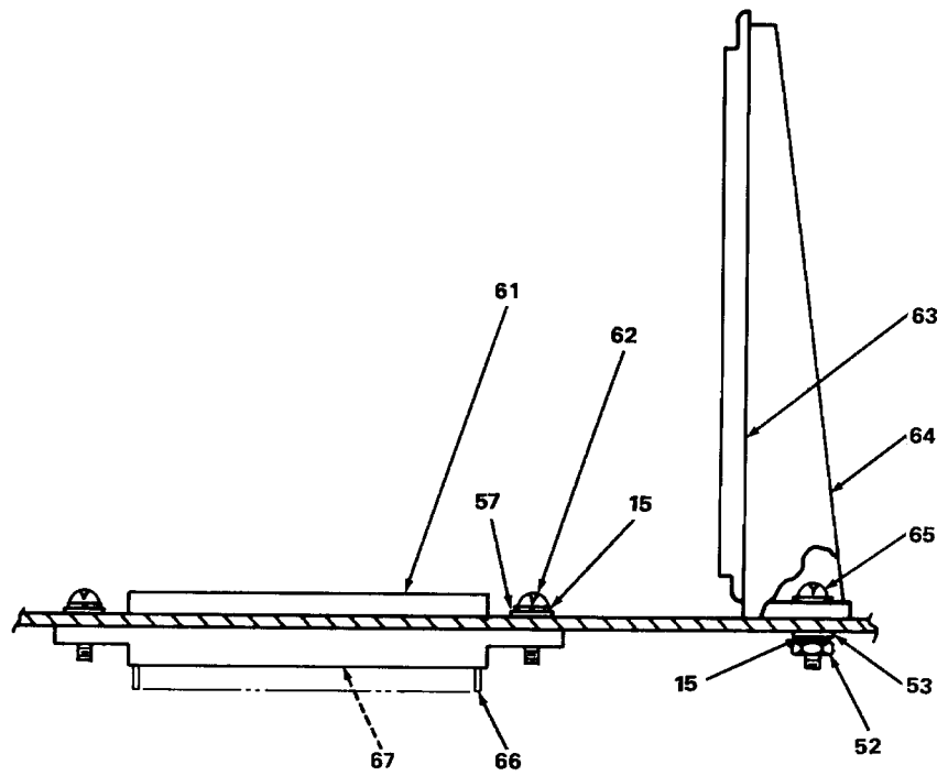
SECTION L-L
