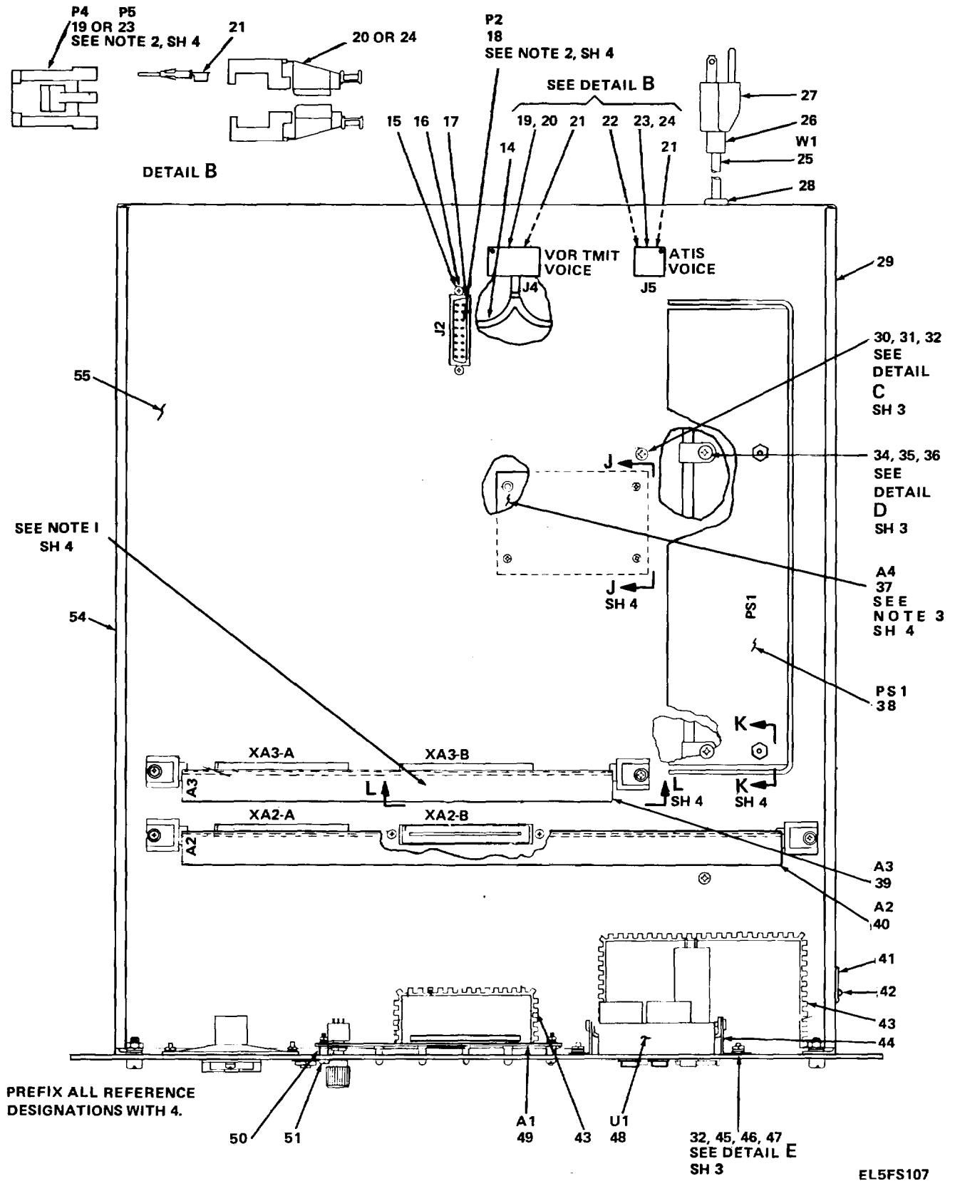
Figure 43. Control-Indicator (Unit 4) C-10526/FRN-41(V) (Sheet 2 of 5).
