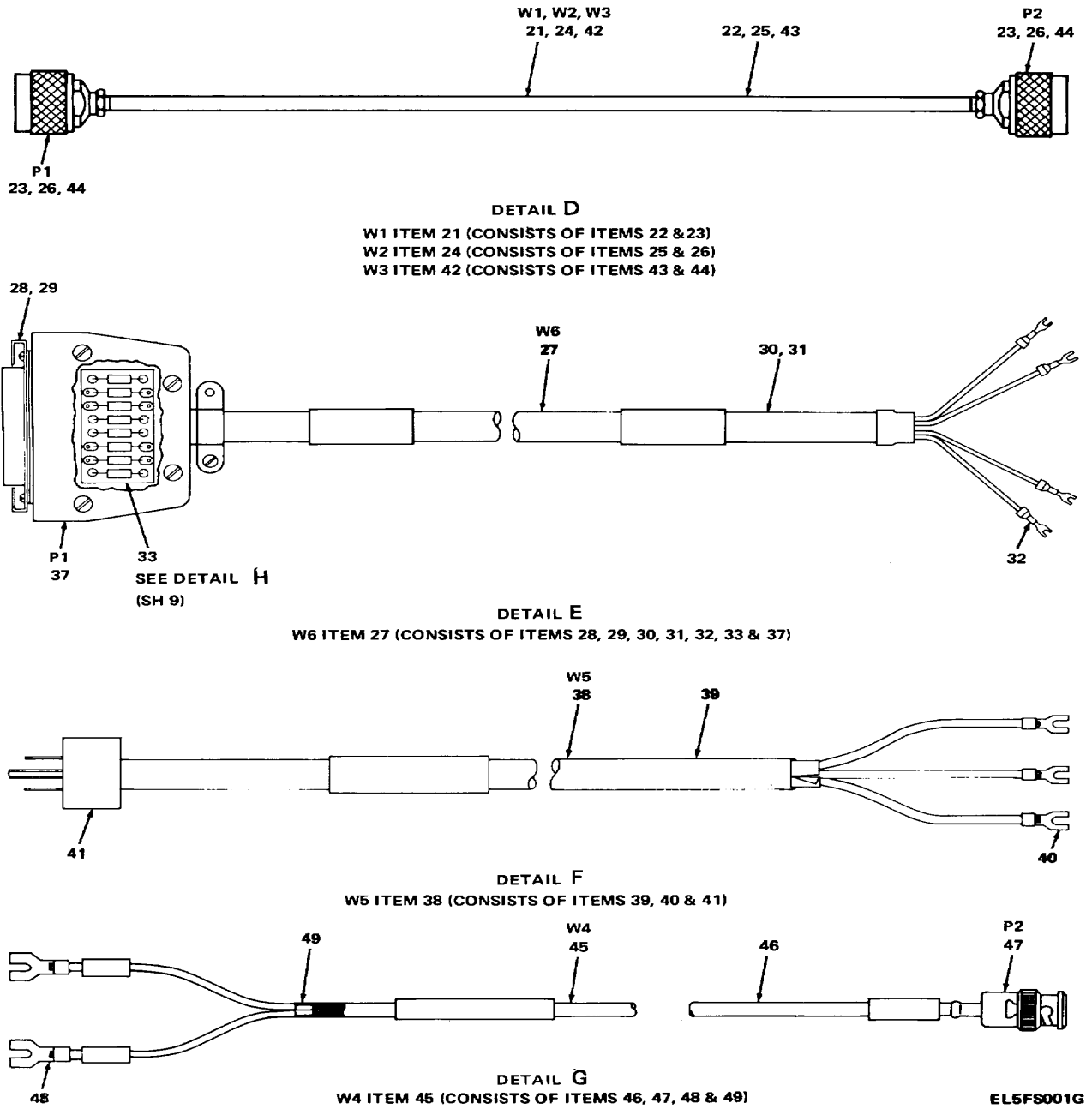
Figure 1. Radio Transmitting Set AN/FRN-41(V) 1,2,3 and 4 and Radio Transmitting Training Set AN/FRN-41(V) T1 (Sheet 5 of 9).
