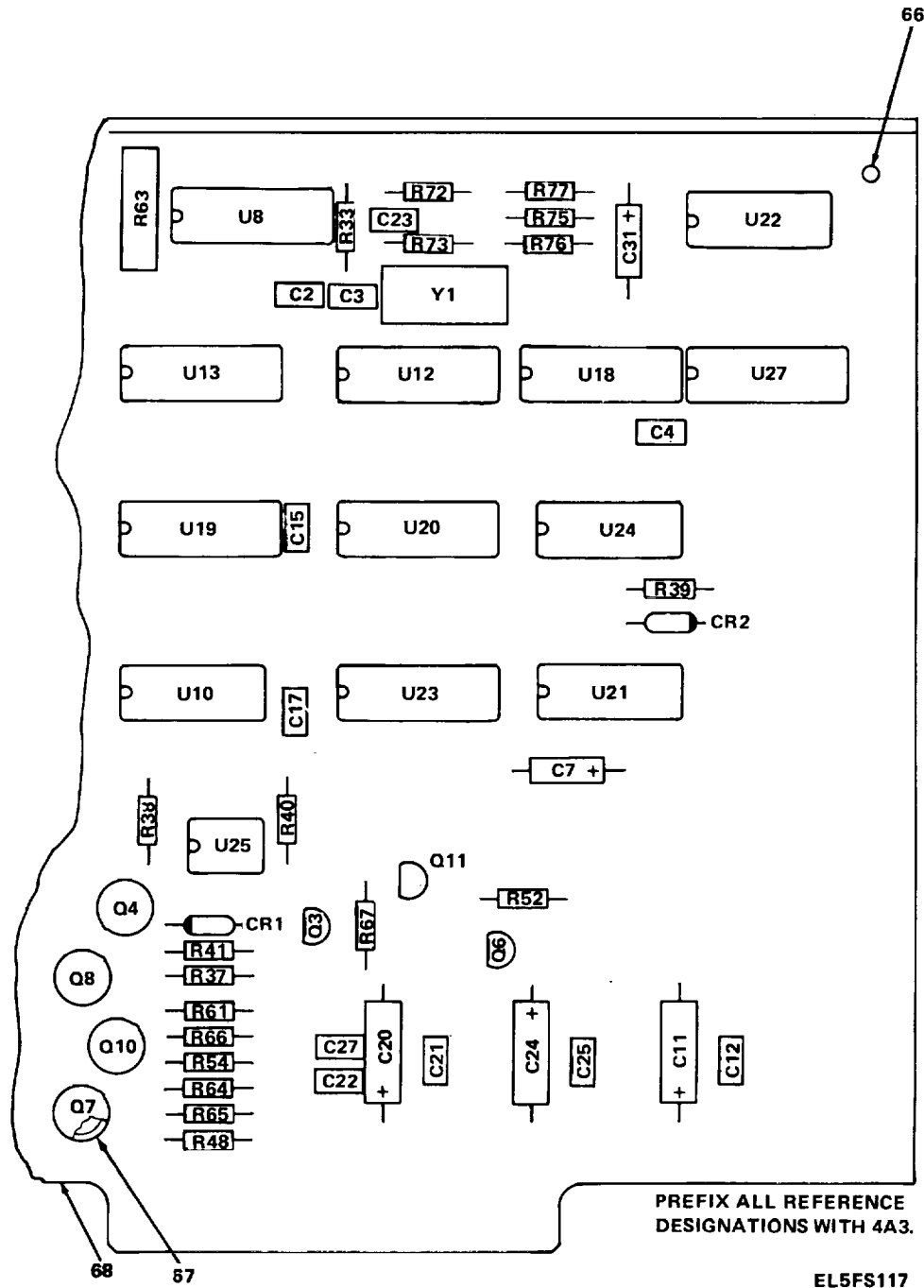
Figure 46. Operation Site (Remote) Modem Circuit Card Assembly (4A3) (Sheet 2 of 3).
