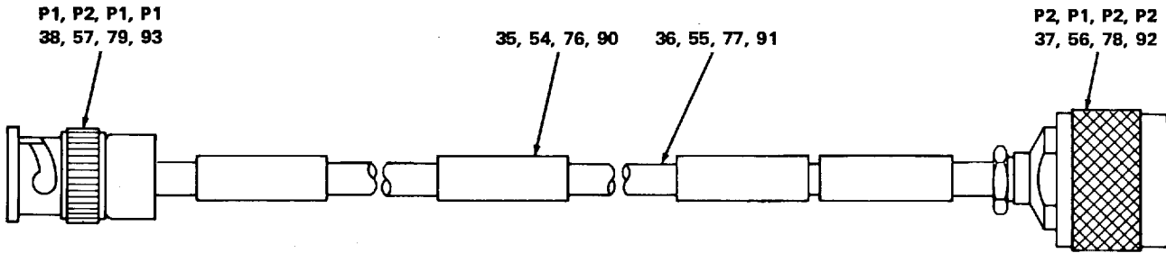
DETAIL E
