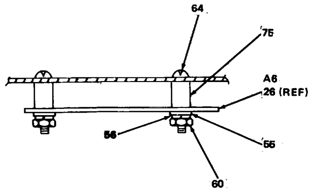
SECTION N-N (ROTATED 90° CW)
