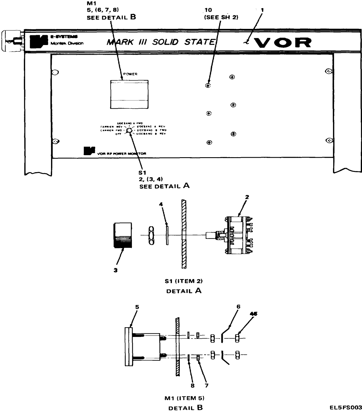
Figure 3. Electrical Equipment Rack (1A1) MT-6011/FRN-41(V) and MT-6134/FRN-41(V) (Sheet 1 of 11).
