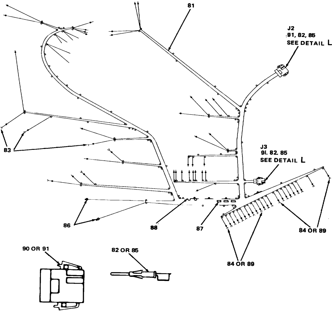
DETAIL L
