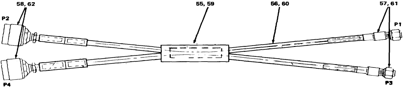
DETAIL M ITEM 55 (W8) CONSISTS OF ITEMS 56, 57 & 58 ITEM 59 (W6) CONSISTS OF ITEMS 60, 61 & 62
