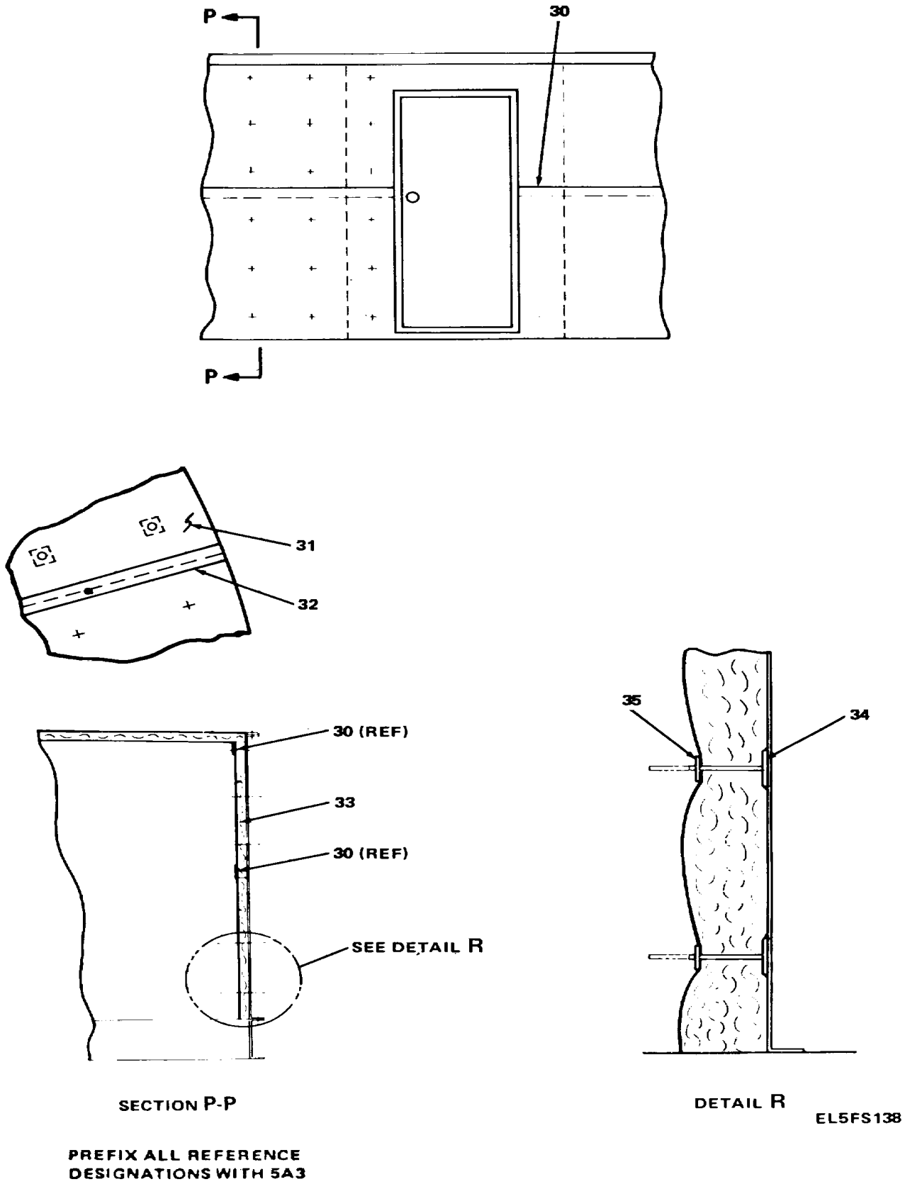
Figure 54. Shelter (5A3) (Sheet 6 of 6).
