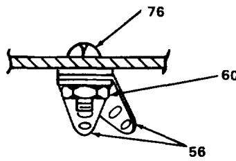
SECTION K-K
