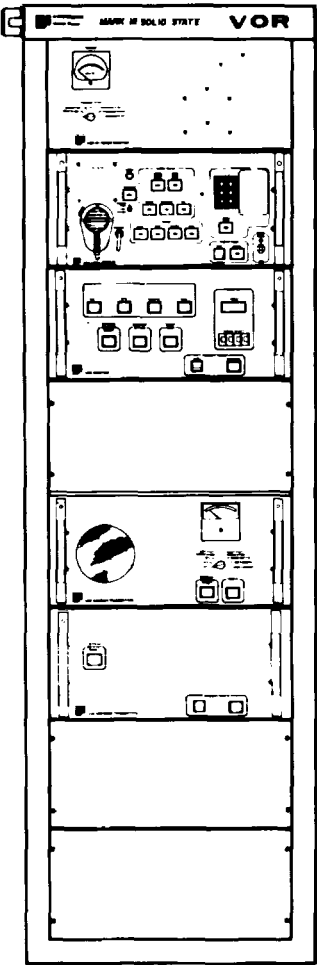
UNIT 1 TRANSMITTER GROUP OT-117/FRN-41(V)
