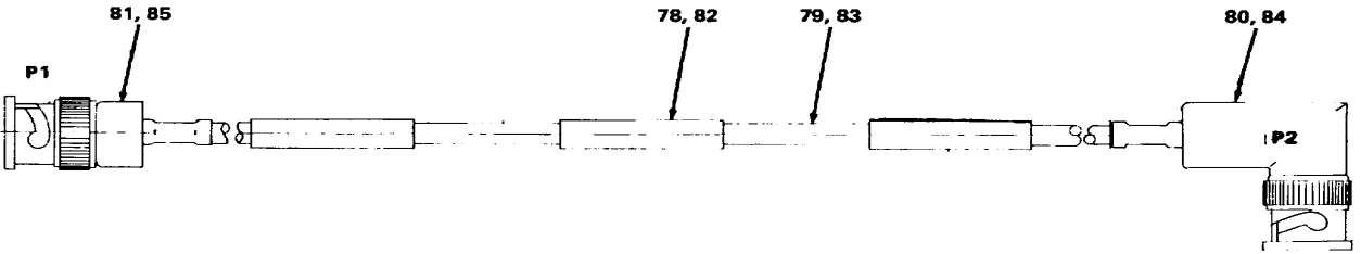
DETAIL S ITEM 78 (W2) CONSISTS OF ITEMS 79, 80 & 81 ITEM 82 (W4) CONSISTS OF ITEMS 83, 84 & 85
