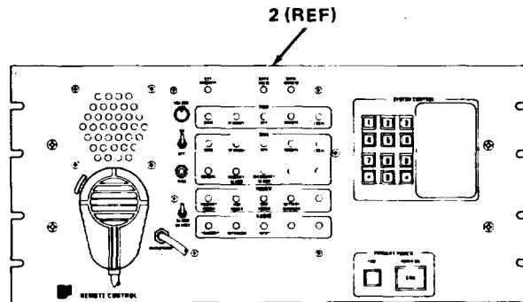
UNIT 4 CONTROL-INDICATOR C-10526/FRN-41(V)
