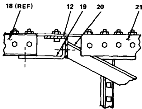
DETAIL F
