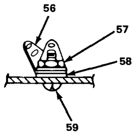
SECTION L-L
