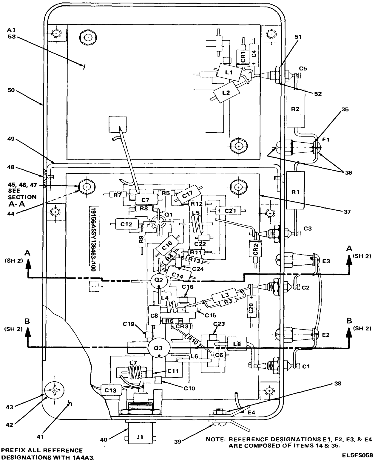
Figure 21. Oscillator/Exciter Assembly (1A4A3/1A7A3) (Sheet 1 of 2)
