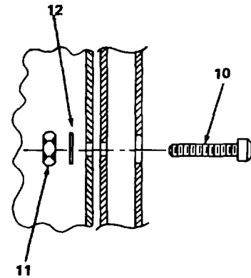
DETAIL E
