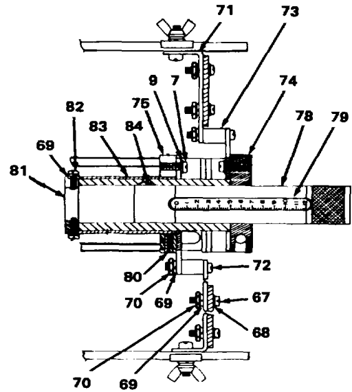
SECTION J-J
