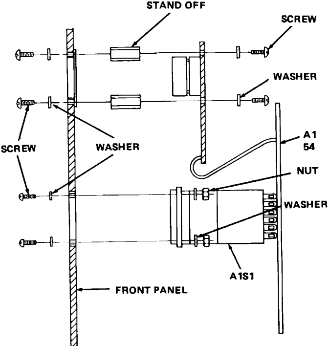
DETAIL E
