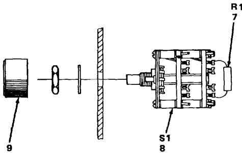
DETAIL B
