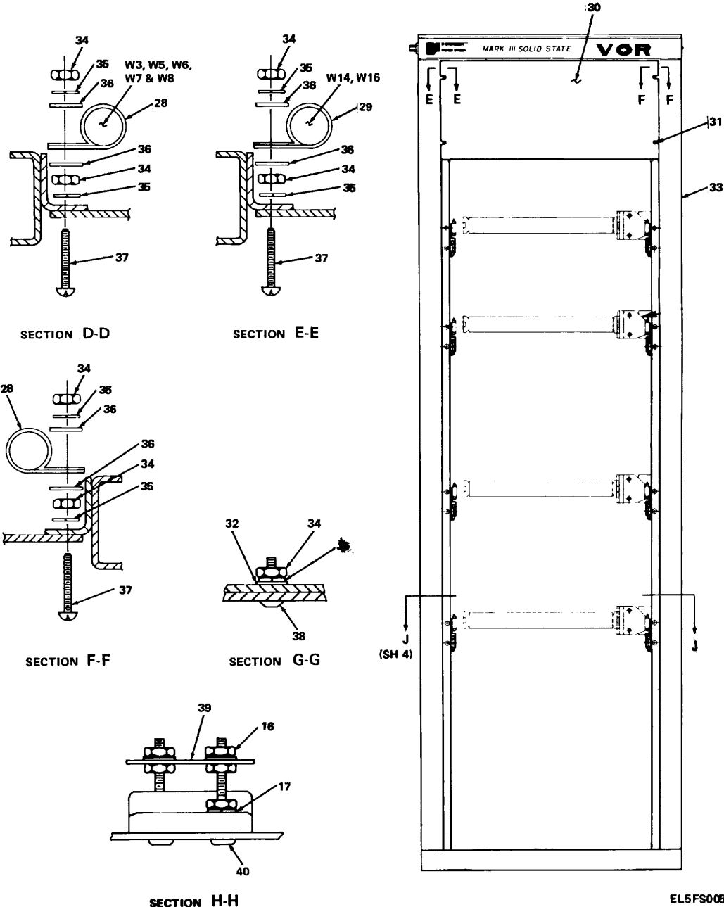
Figure 3. Electrical Equipment Rack (1A1) MT-6011/FRN-41(V) and MT-6134/FRN-41(V) (Sheet 3 of 11).
