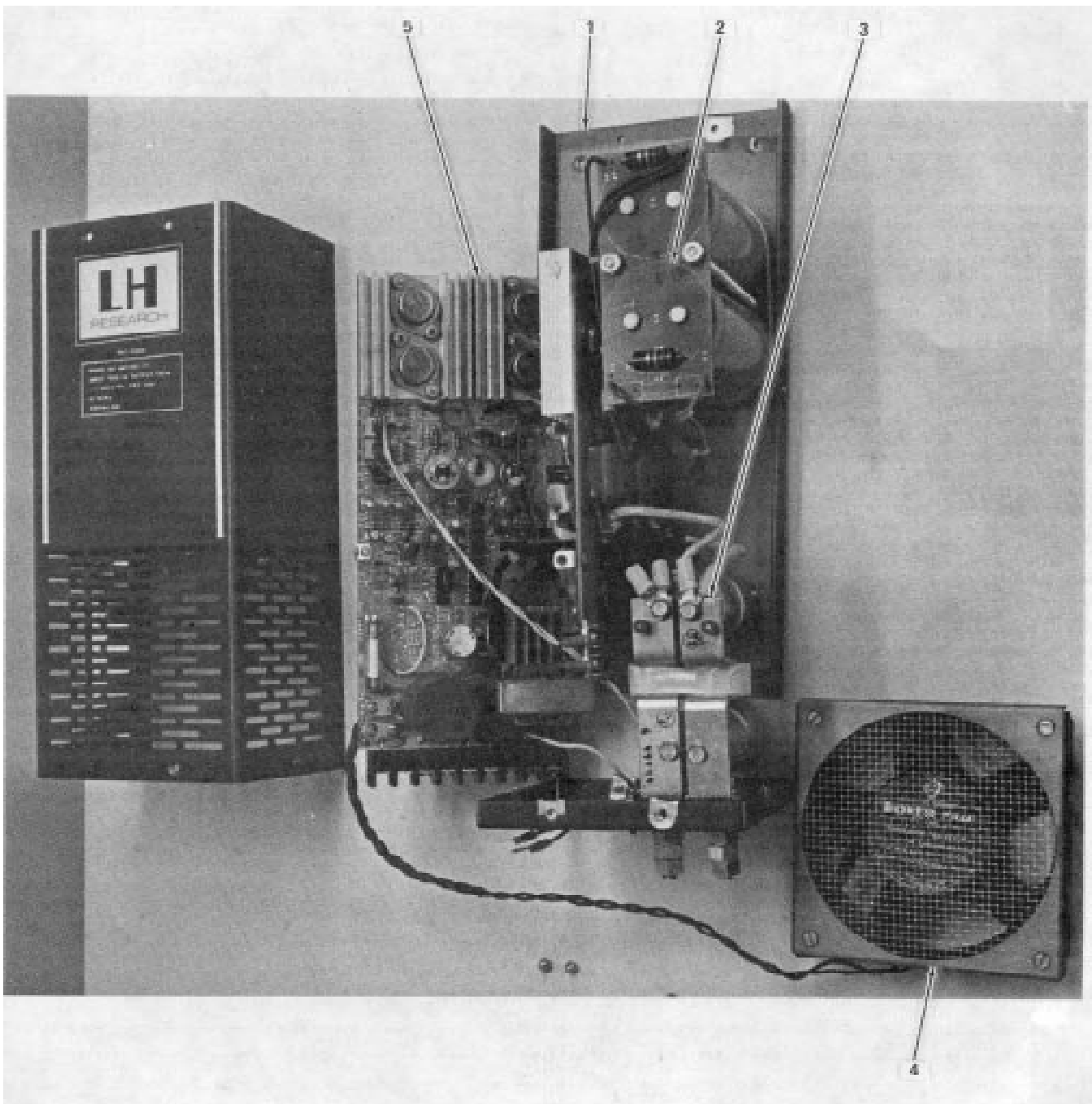
Figure 27. Power Supply (1a4ps1/1a7psi).
