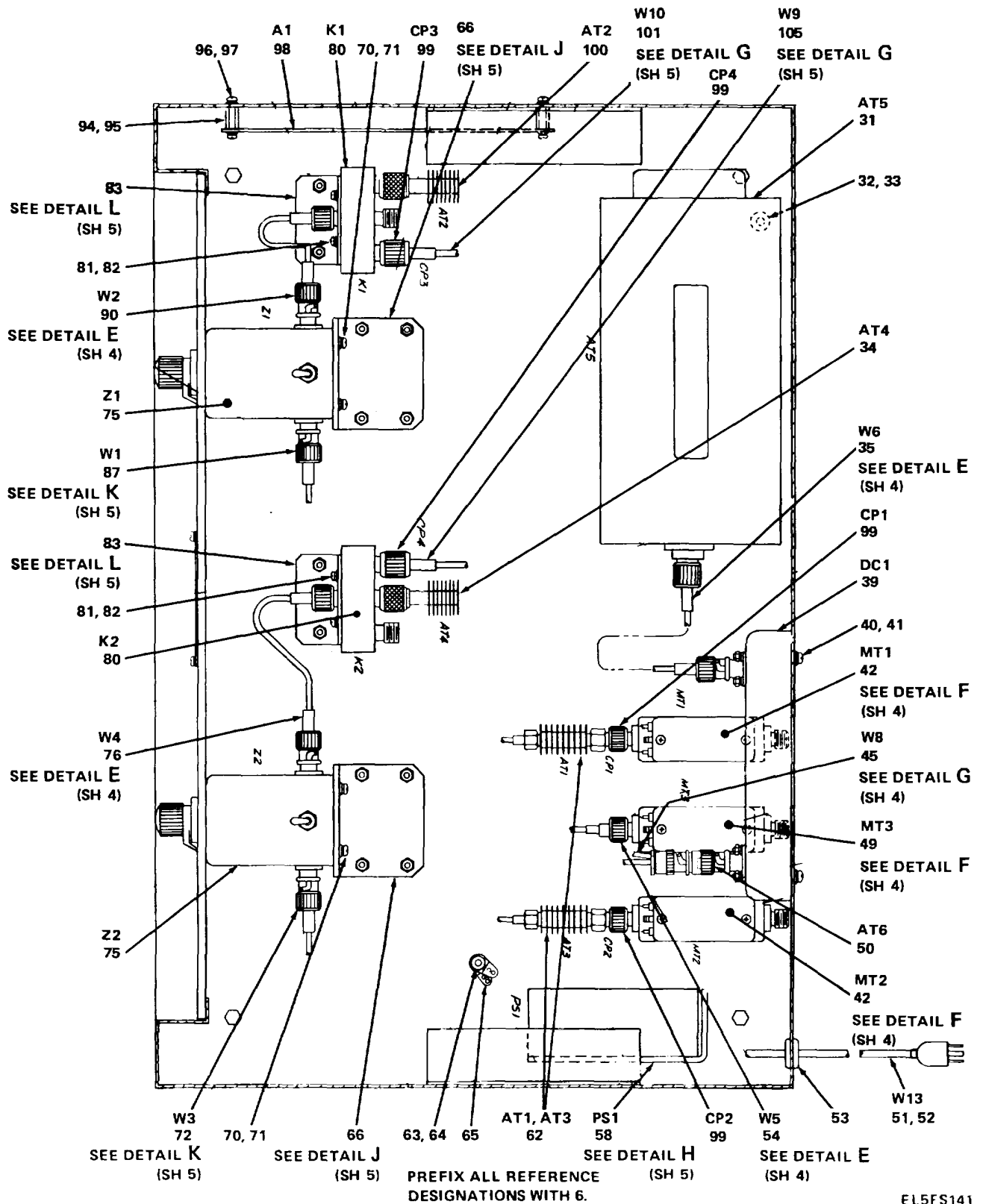
Figure 55. Simulator, Radio Frequency Detector, SM-774/FRN-41(V)T1 (Sheet 3 of 5).
